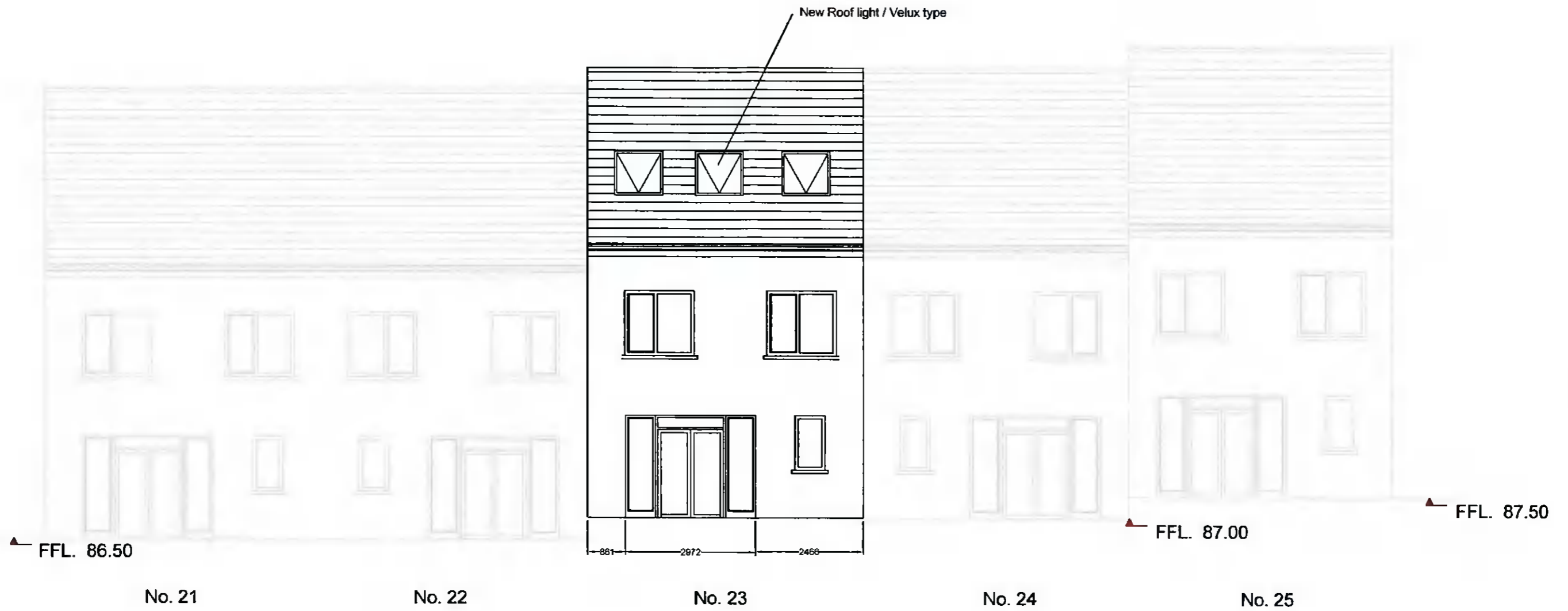
Proposed Rear Elevation Scale 1:100
