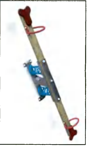
5: Seesaw with springs Provider: Kompan or similar Age Group: 3-8 Materials: Treated timber & steel
