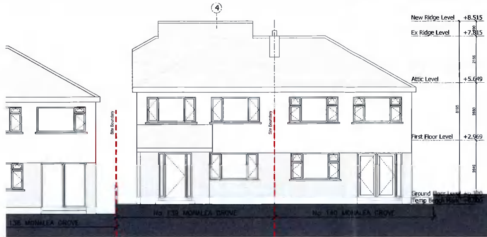
1 Proposed Front/ West Elevation Scale 1:100 @ A3
