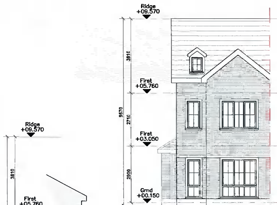
Proposed Front Elevation Scale 1/100 (No Change)
