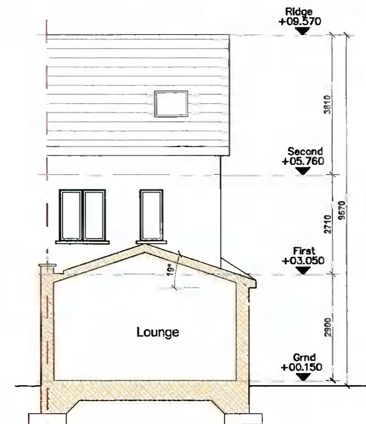
Proposed Typical Section Scale 1/100
