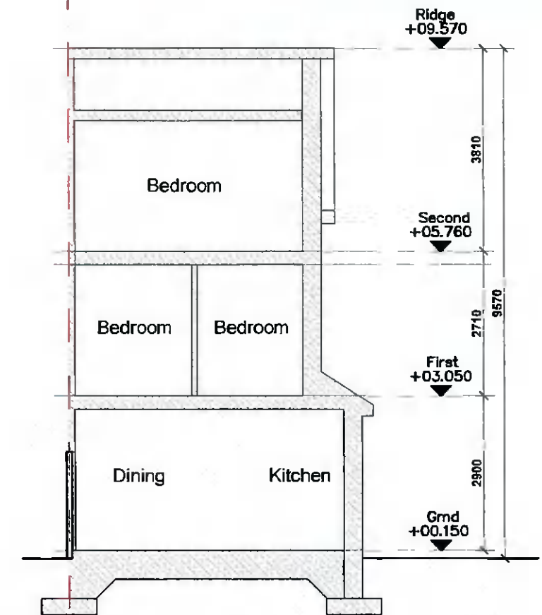
Existing Typical Section Scale 1/100
