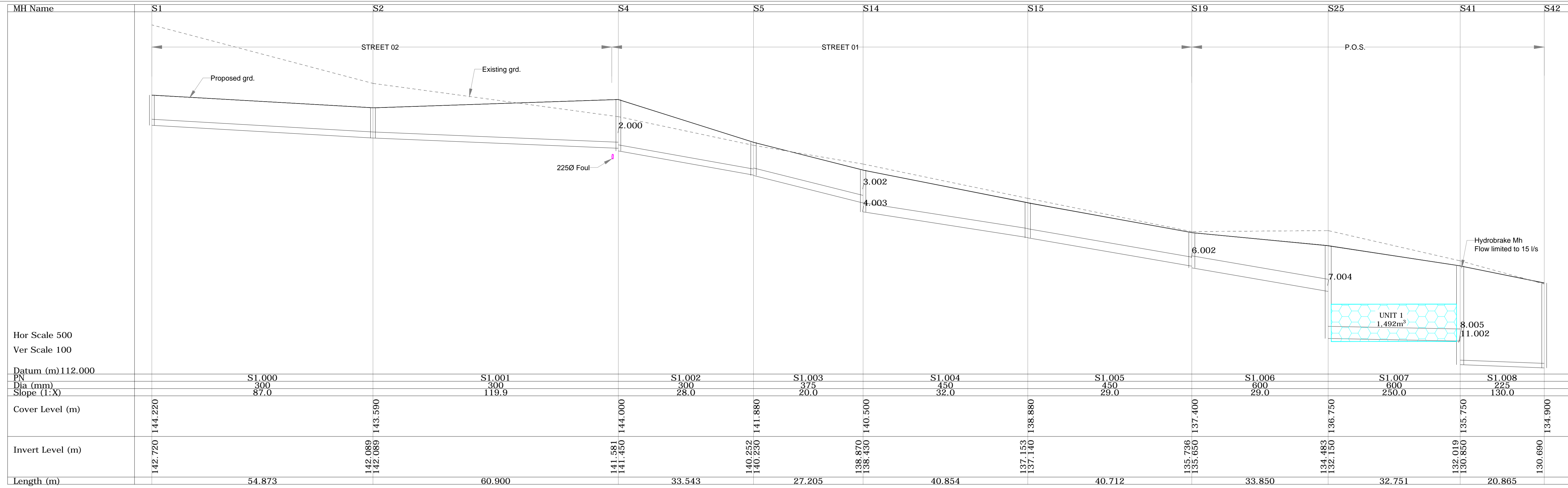
S/W Longitudinal Section S1 to S42
