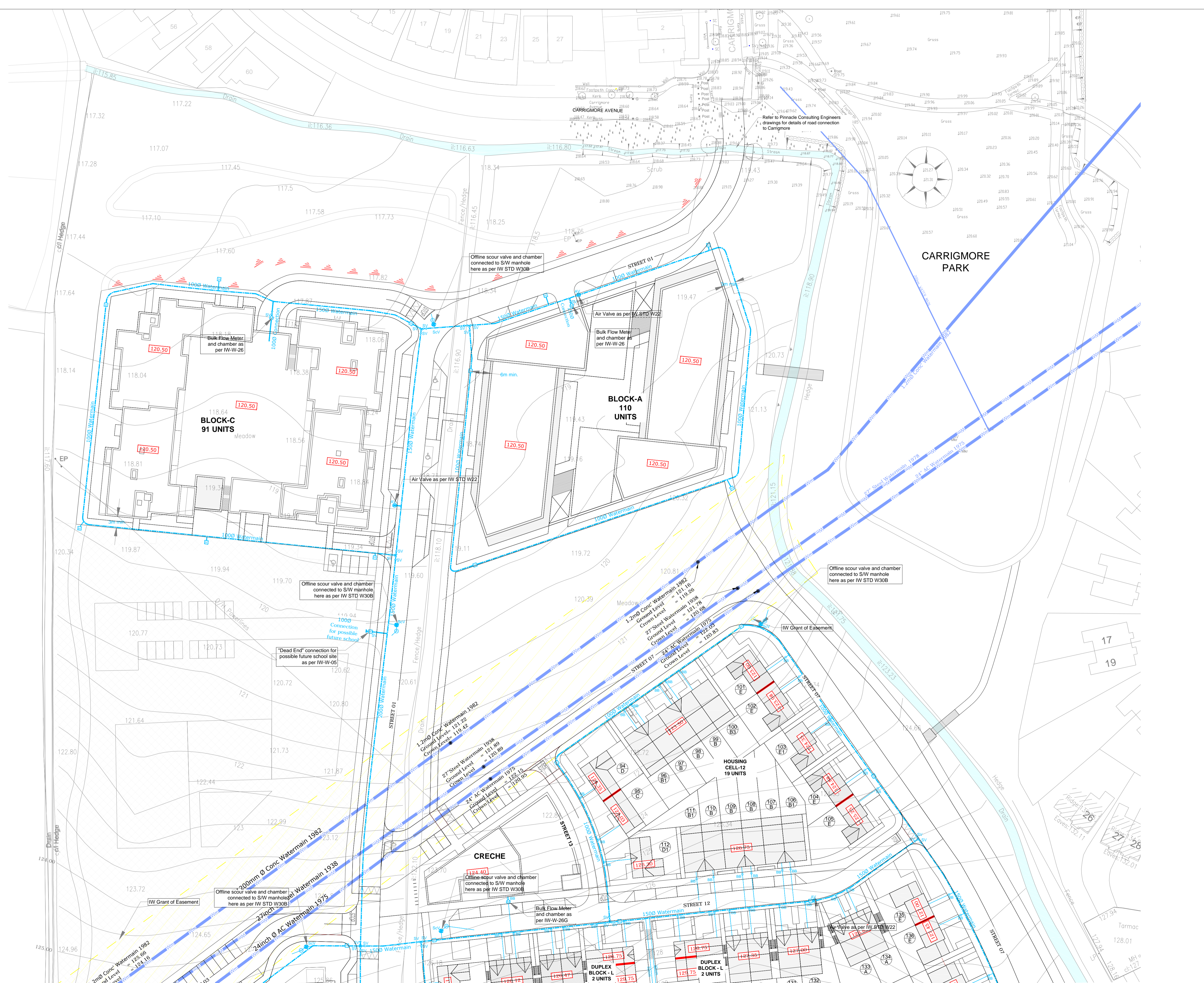
Watermain GA © A1 - Scale 1:500
