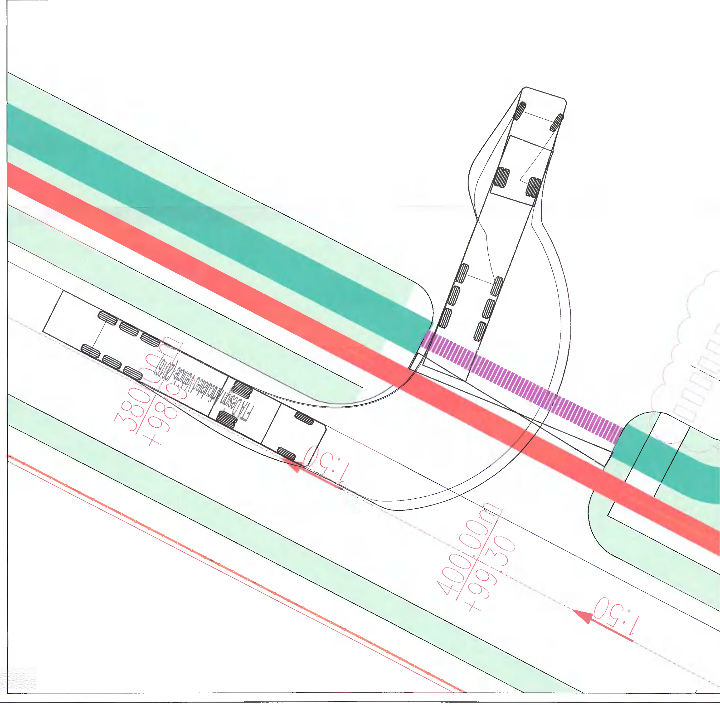
HGV - SITE B2 ACCESS - SCALE 1:100
