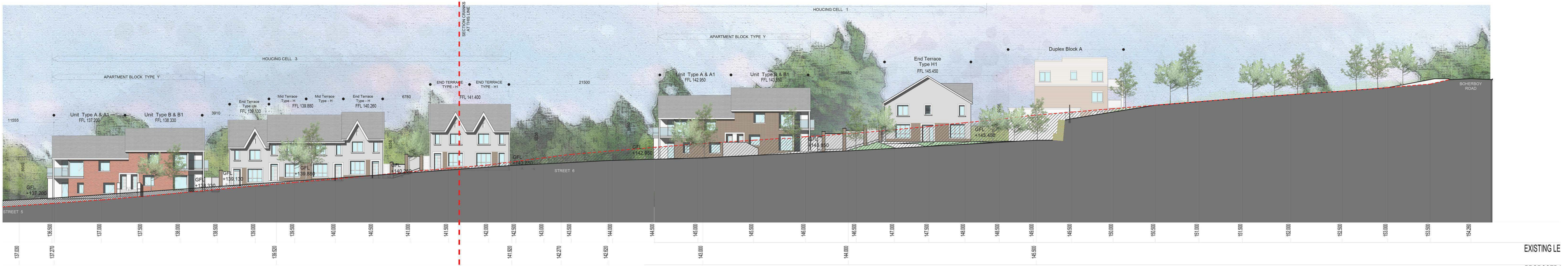
LONG SECTION X-X (PART 1) - LOOKING WEST Scale 1:200
