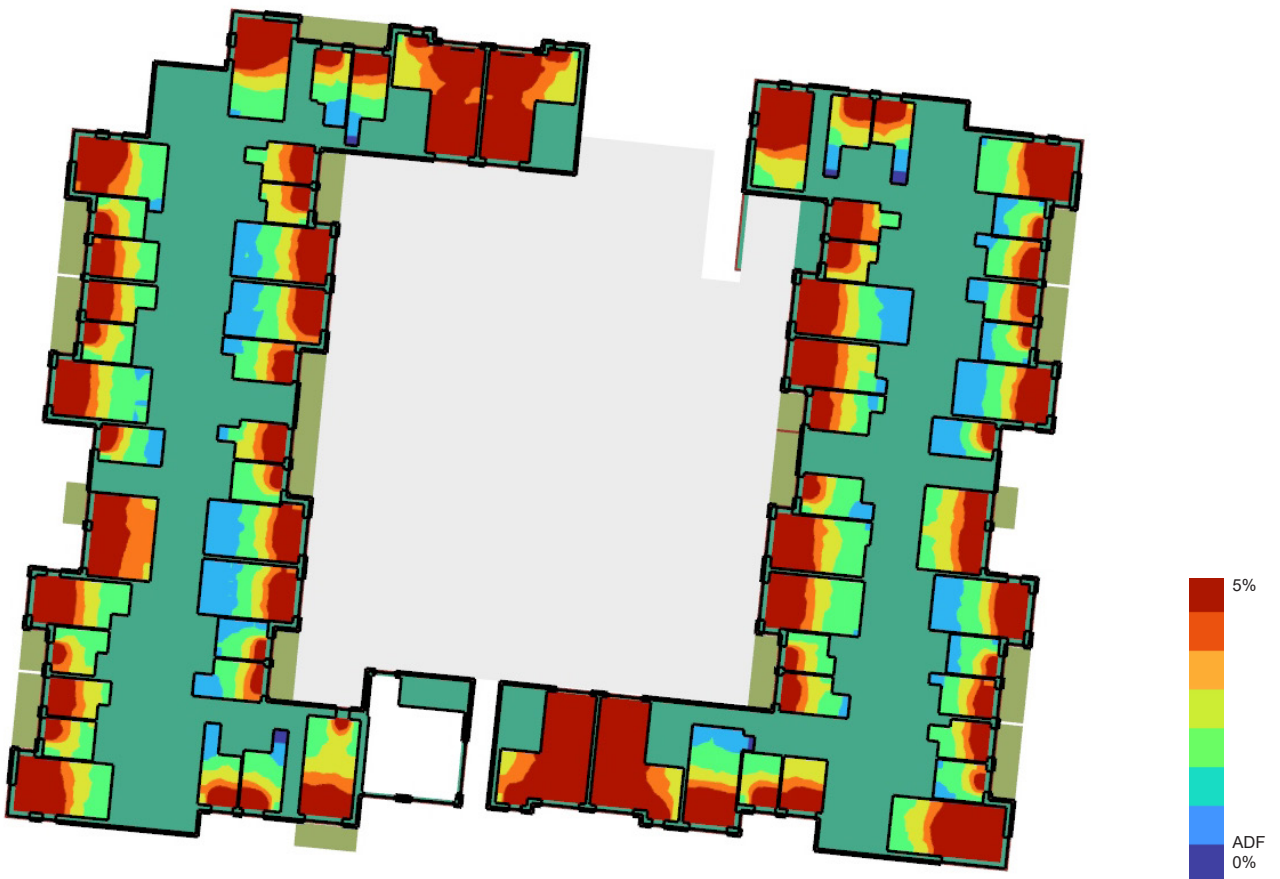
Figure 33: Block C - First floor false colour plan of ADF. Scale 0 - 5%
