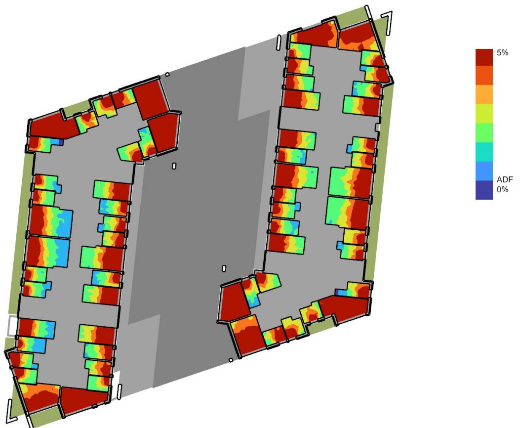
Figure 28: Block A - First floor false colour plans of ADF. Scale 0 - 5%
