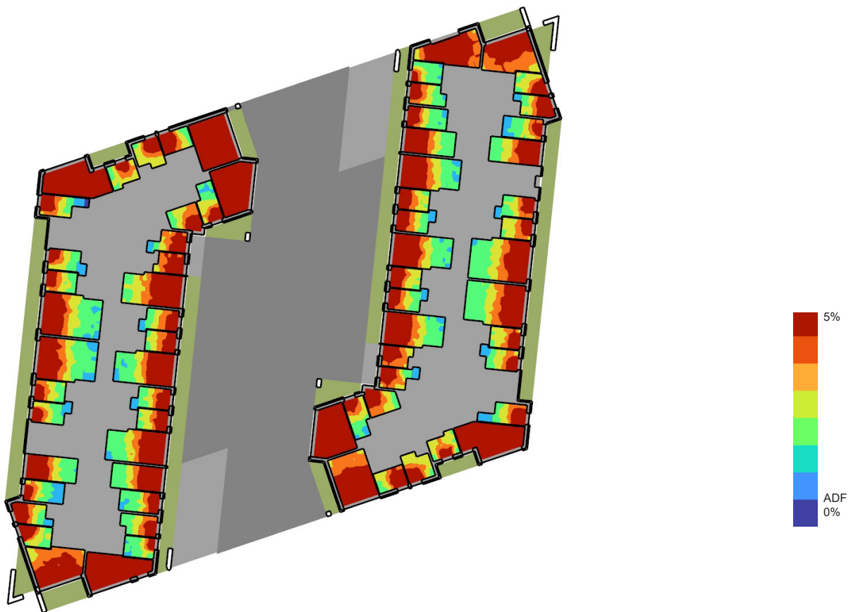
Figure 29: Block A - Third floor false colour plans of ADF. Scale 0 - 5%
