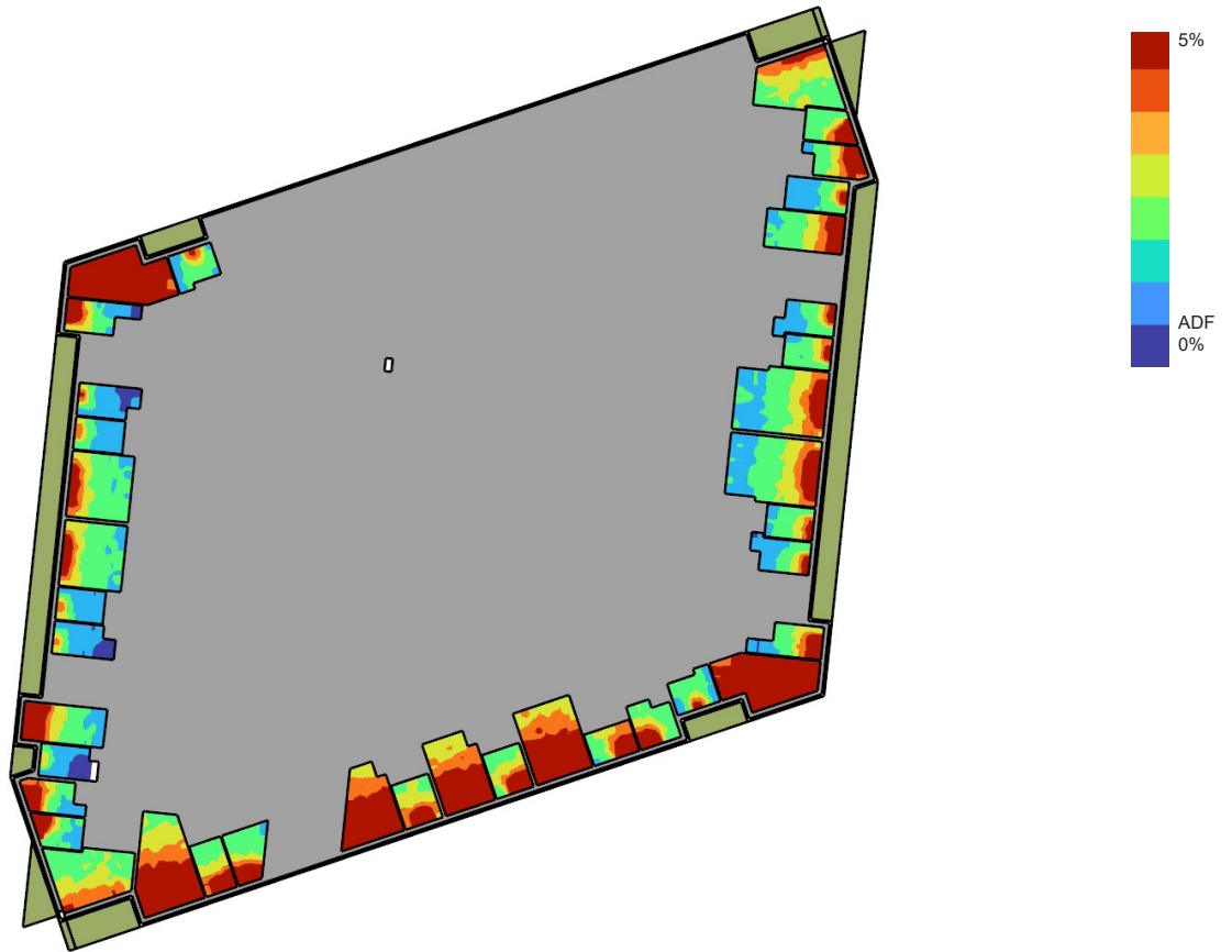
Figure 27: Block A - Ground floor false colour plans of ADF. Scale 0 - 5%
