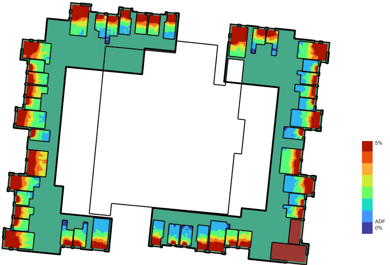
Figure 34: Block C - Ground floor false colour plan of ADF. Scale 0 - 5%
