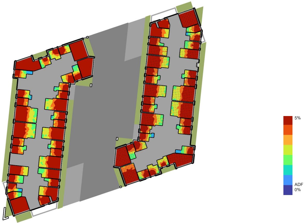
Figure 31: Block A - Fourth floor false colour plans of ADF. Scale 0 - 5%
