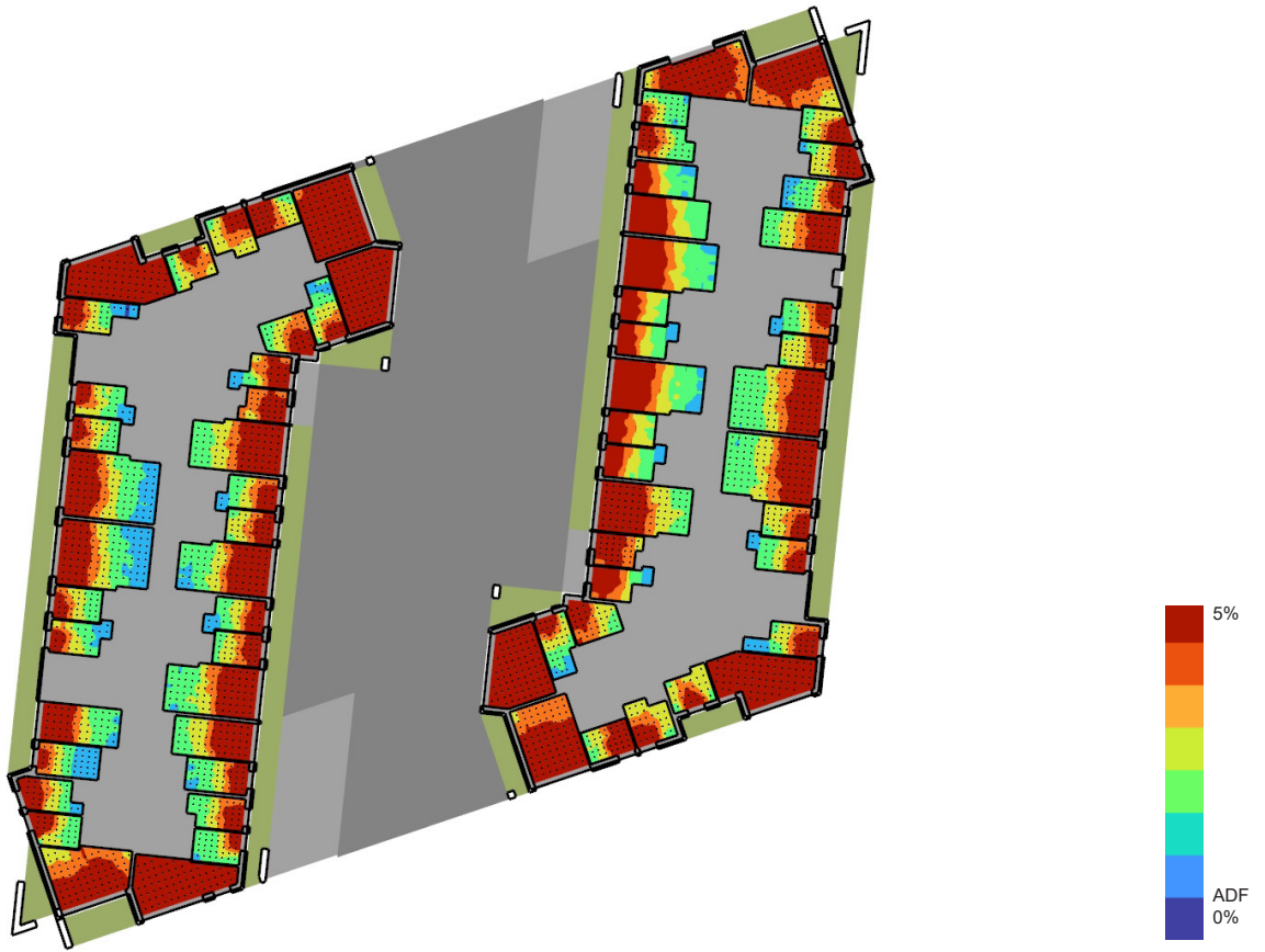
Figure 30: Block A - Second floor false colour plans of ADF. Scale 0 - 5%
