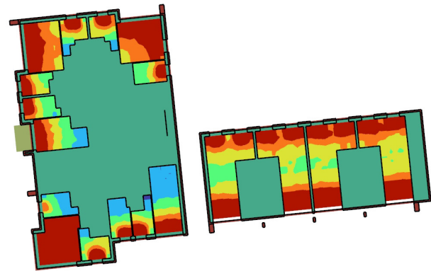
Figure 32: Block B - All floors false colour plans of ADF. Scale 0 - 5%
