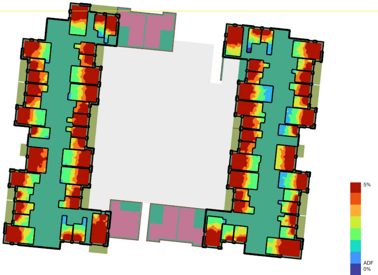
Figure 36: Block C - Second floor false colour plan of ADF. Scale 0 - 5%
