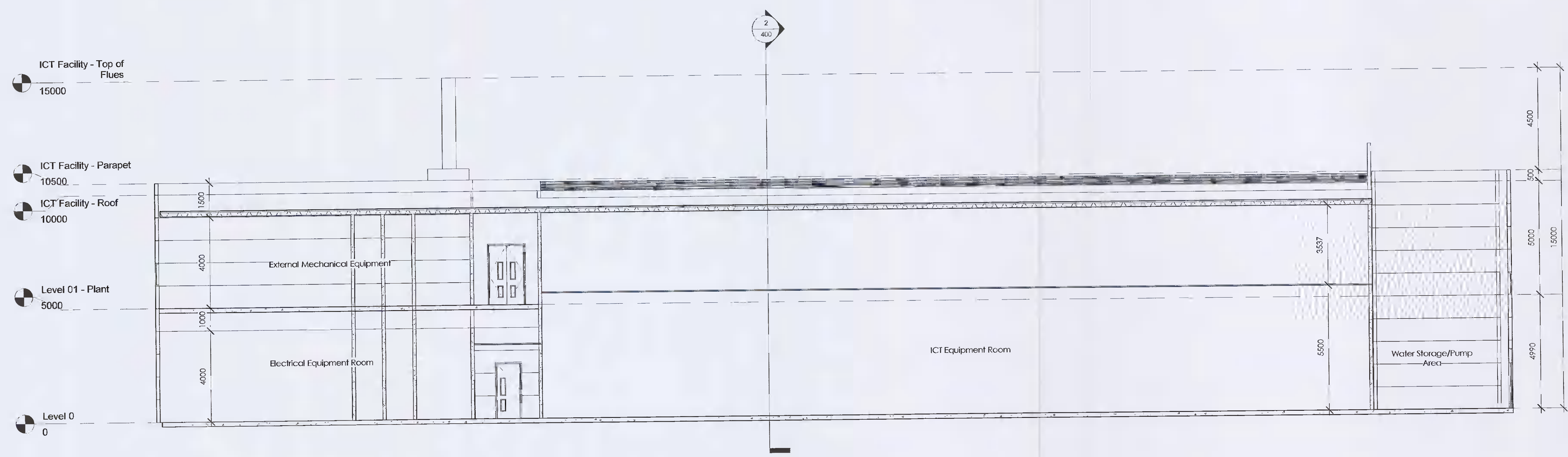
1 Building Section 1 - Permitted 1 : 100
