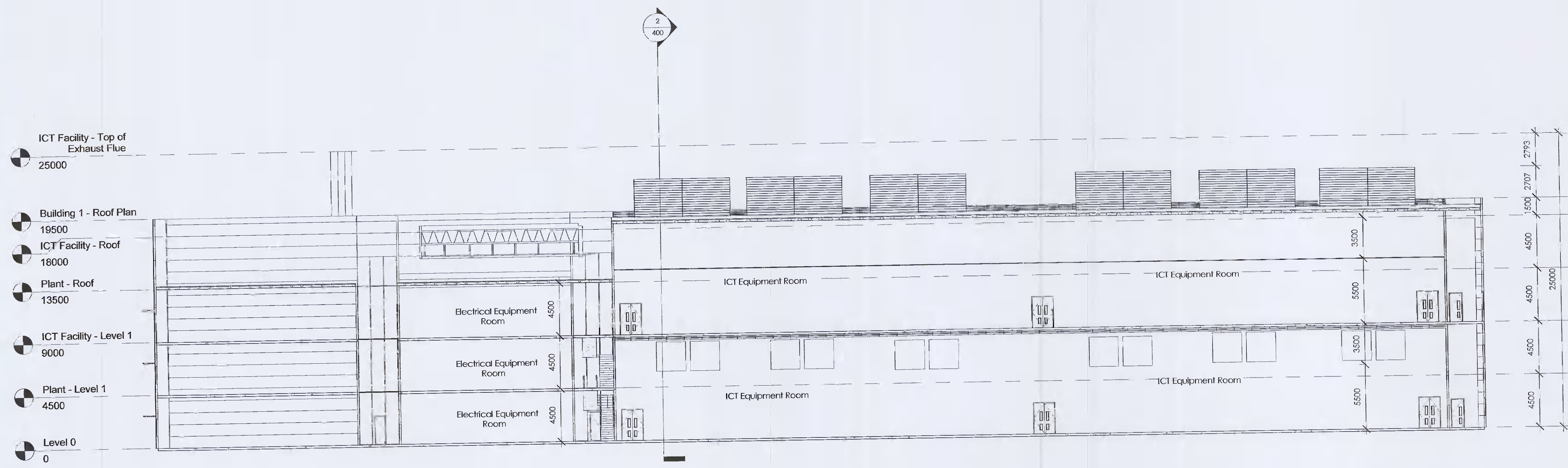
1 Building Section 1 - Permitted 1 : 200
