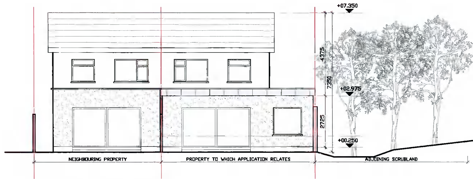
Proposed Rear Contiguous Elevation Scale - 1:100
