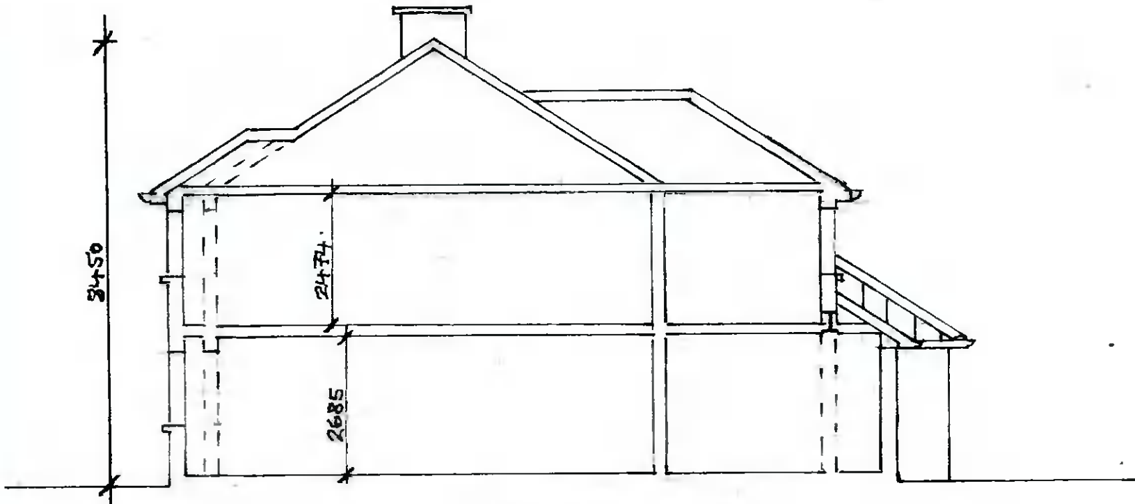
PROPOSED SECTION
