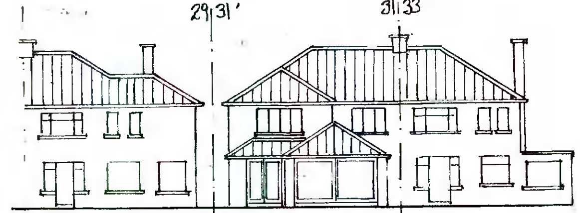
CONTIGUOUS REAR ELEVATION 1:200
