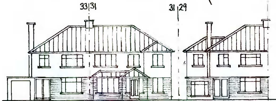
CONTIGUOUS FRONT ELEVATION 1:200
