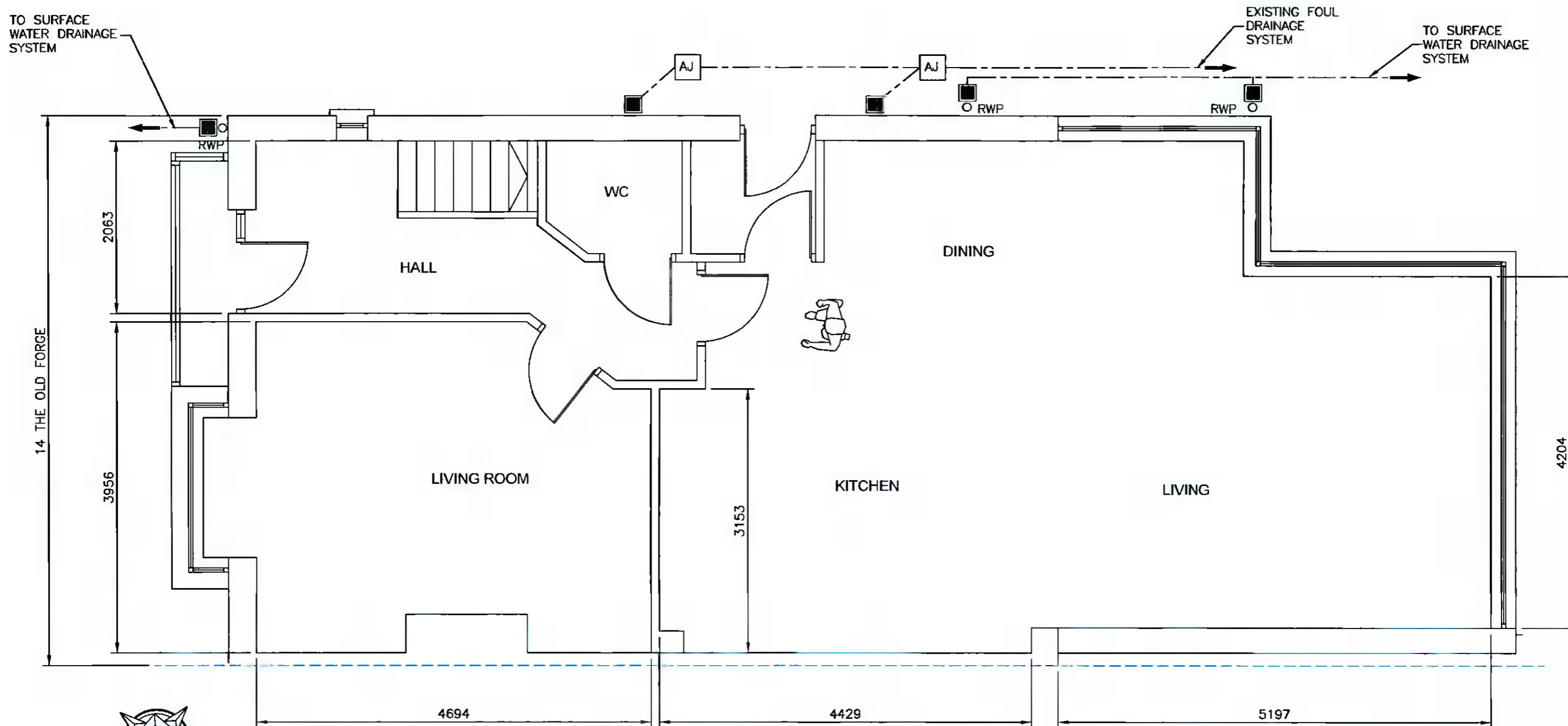
EXISTING GROUND FLOOR PLAN VIEW
