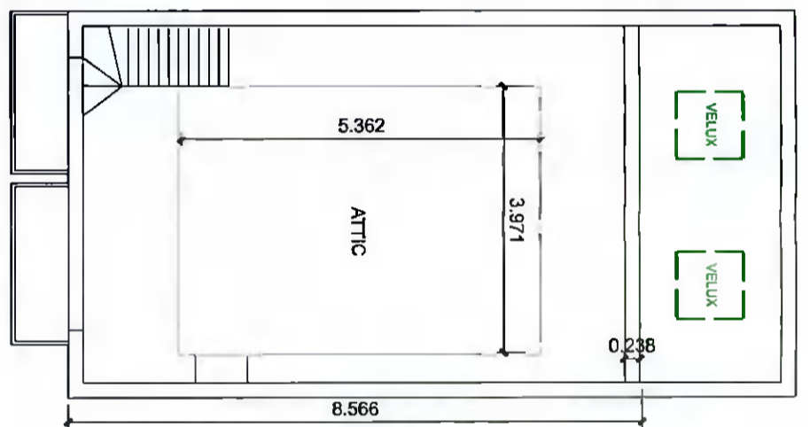
EXISTING ATTIC PLAN
