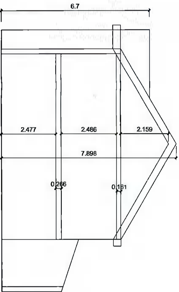
EXISTING CROSS SECTION
