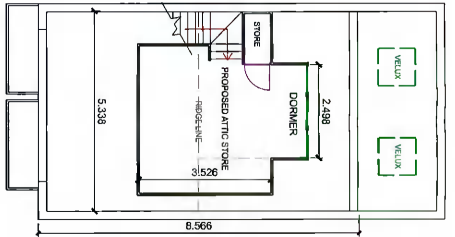
PROPOSED ATTIC PLAN
