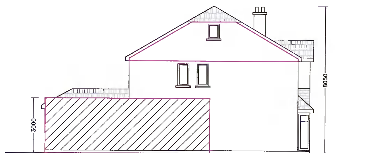
SIDE ELEVATION (PROPOSED) SCALE 1:100
