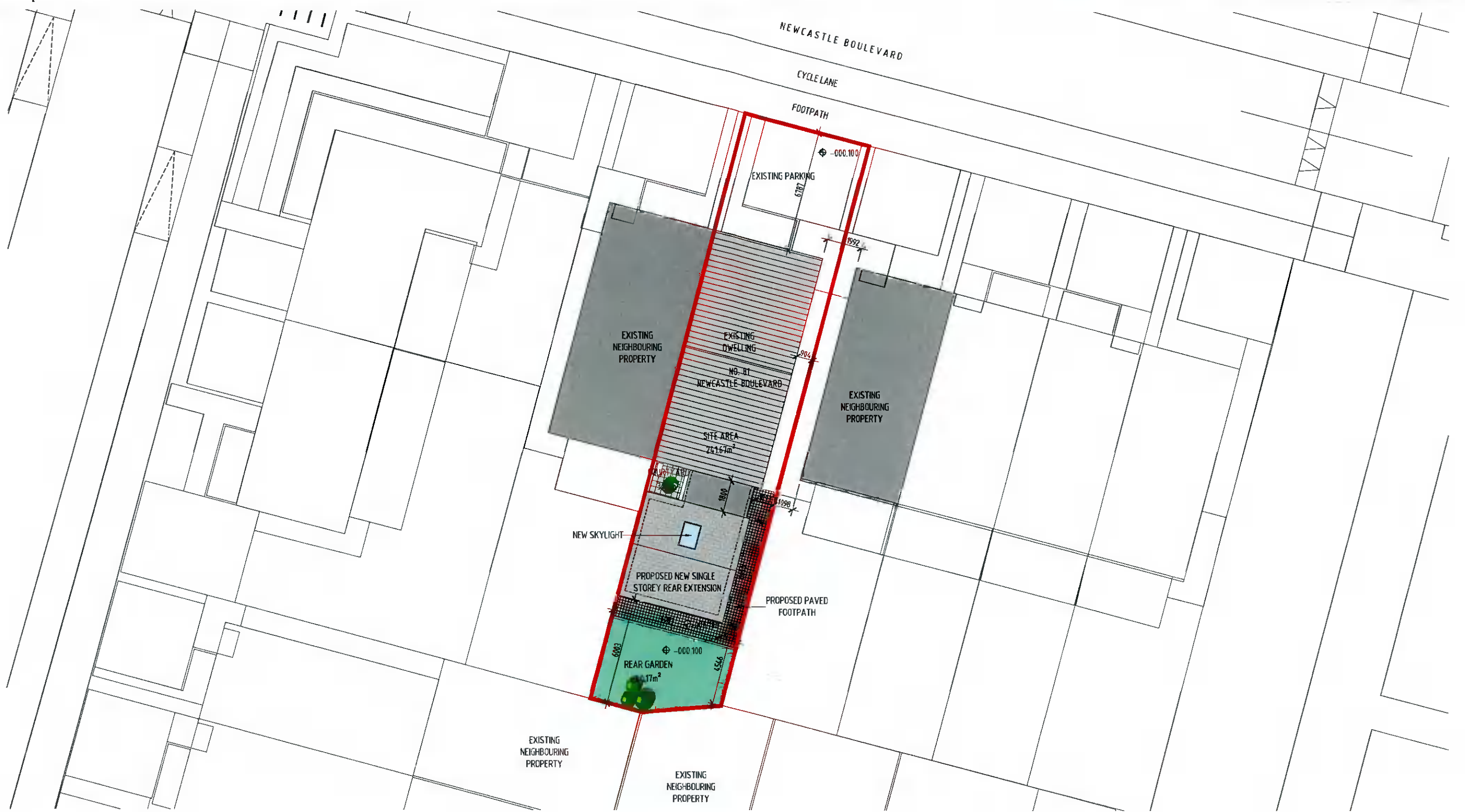
Proposed Site Plan Scale 1:200
