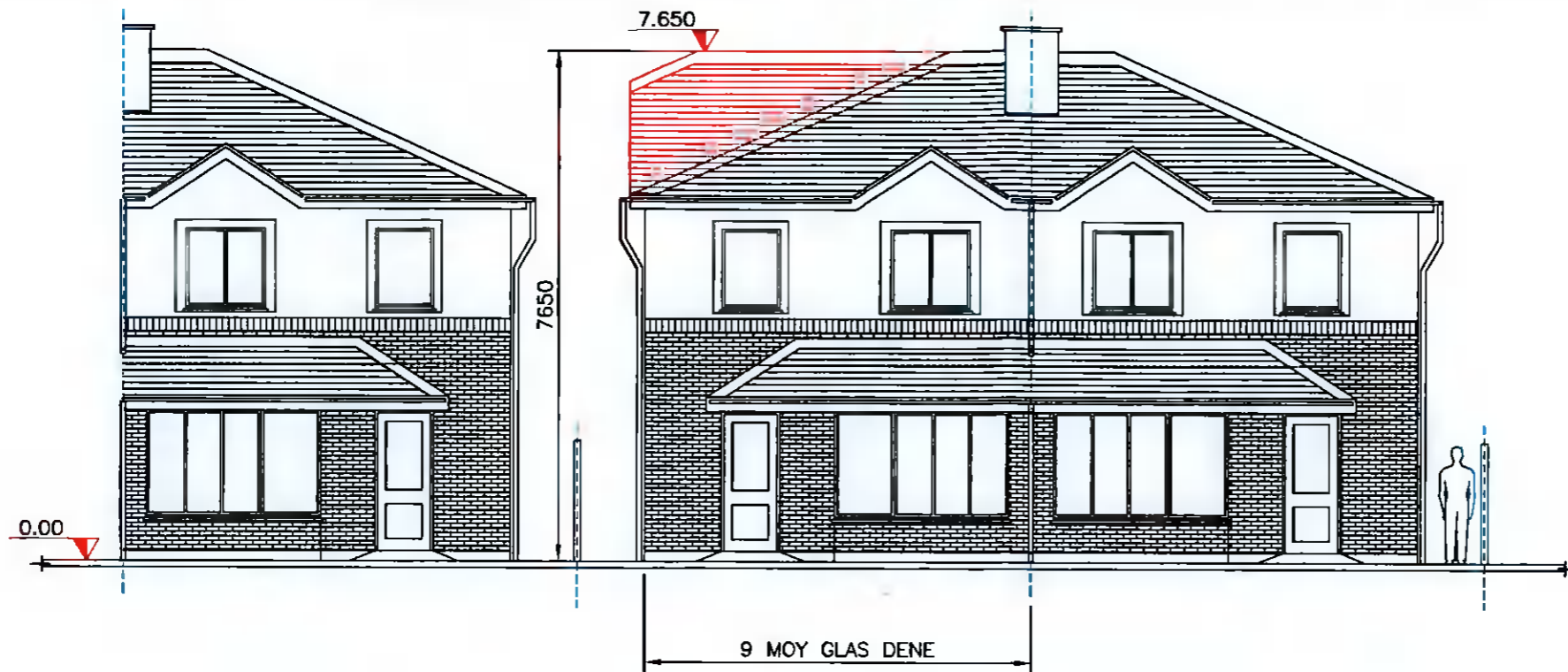
PROPOSED FRONT ELEVATION - CONTIGUOUS
