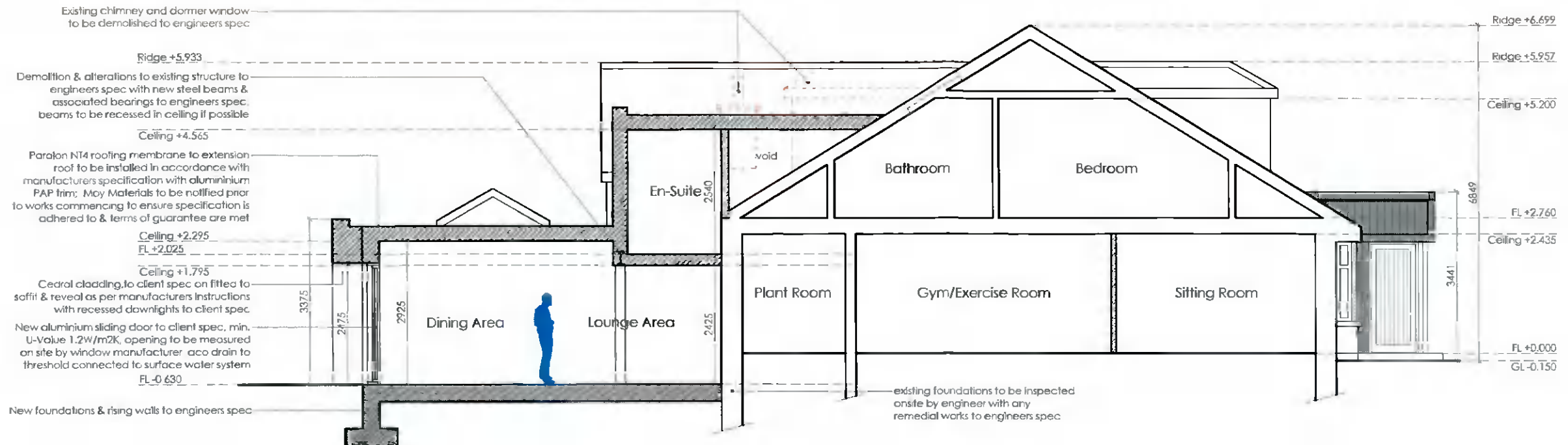
Proposed Section A-A scale 1:100 @ A3
