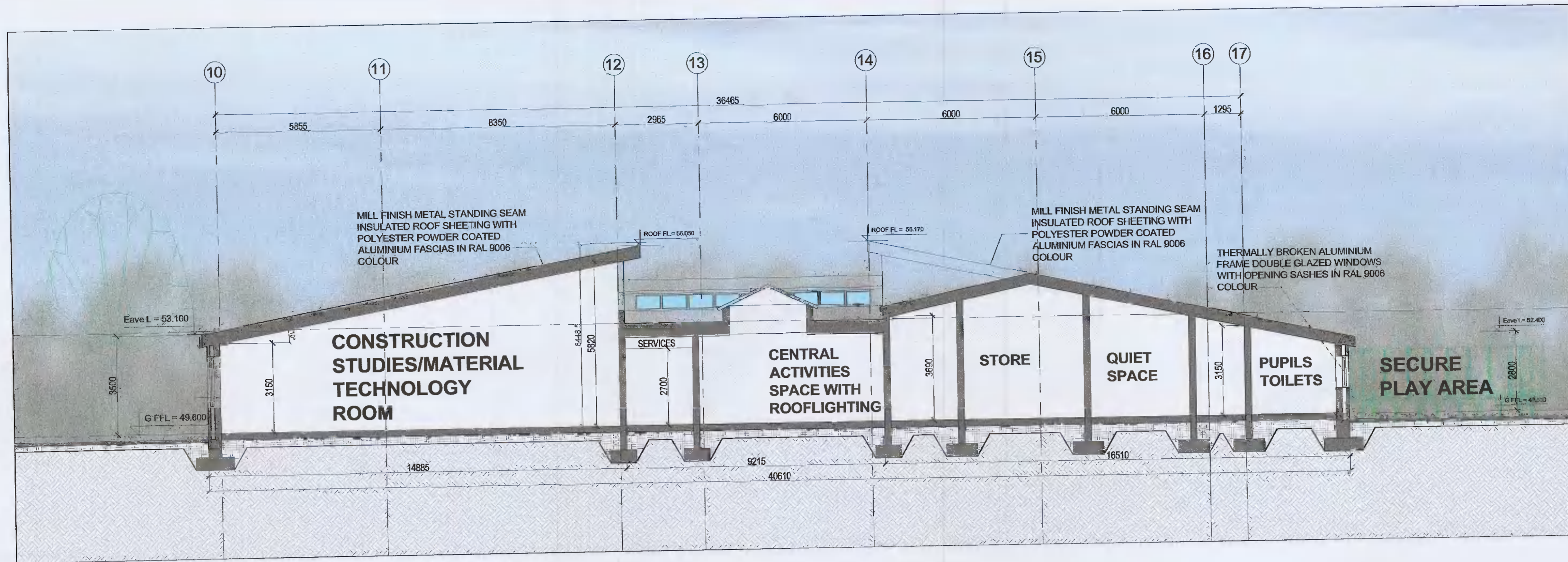
01 SECTION E-E Refer to DR-146 for More Details
