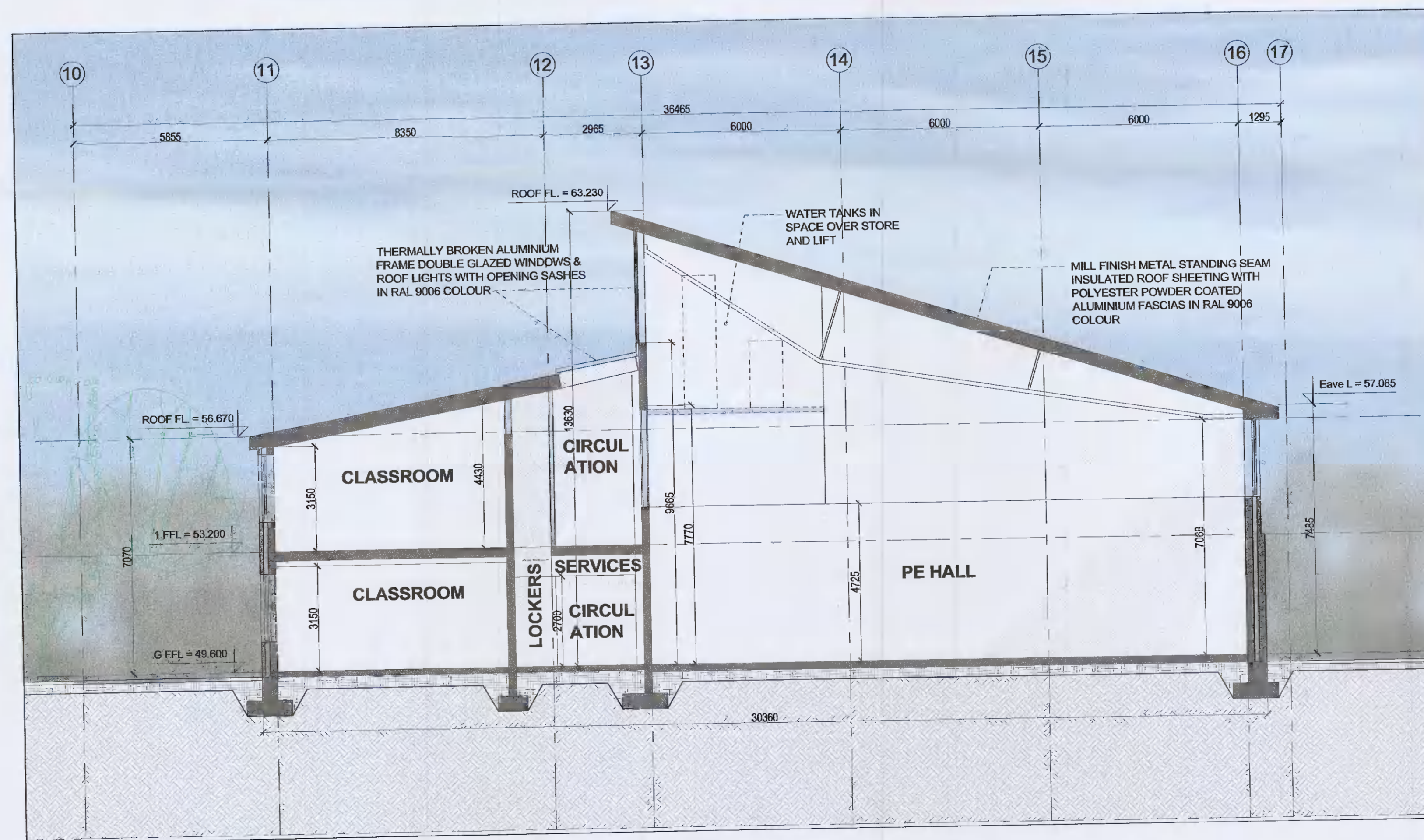
02 SECTION F-F Refer to DR-144 for More Details
