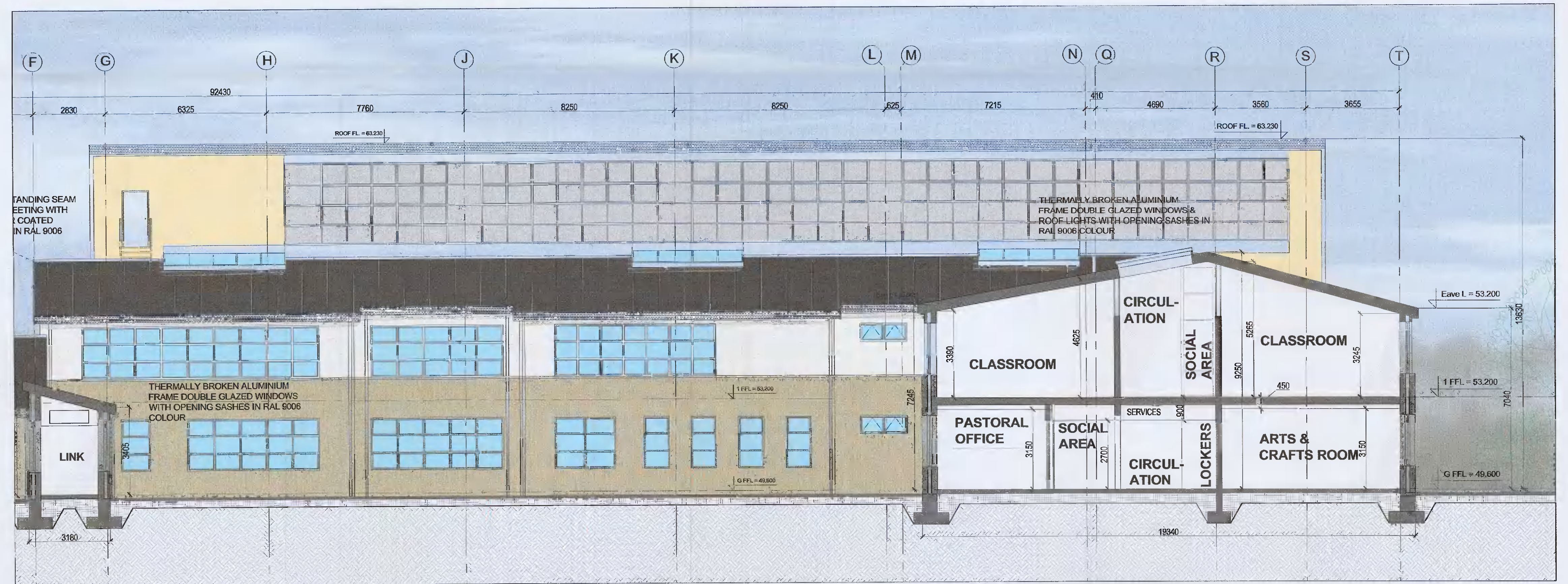
02 SECTION C-C (Part 2)
