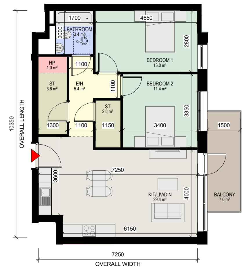
1 Apartment Type 1Y 1 : 100 - 2 BED, 4 PERSON APARTMENT - GROSS INTERNAL AREA (GIA) : 73.29 sqm
