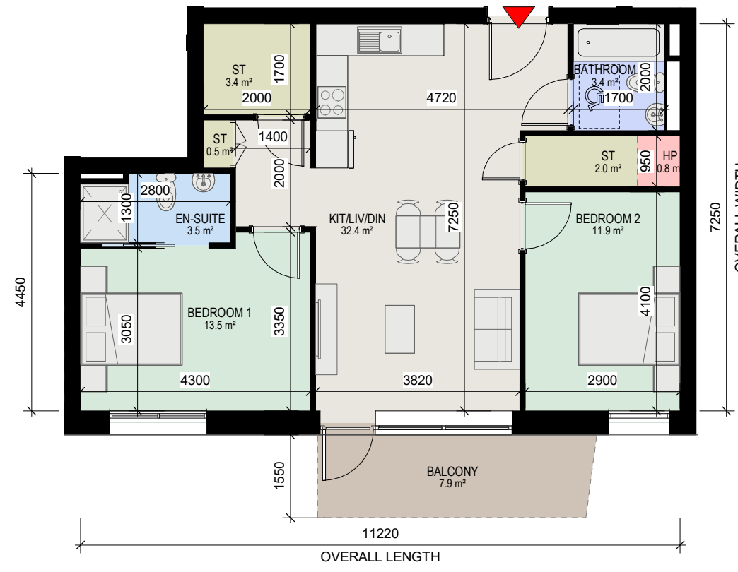
2 Apartment Type 2Z 1 : 100 - 2 BED, 4 PERSON APARTMENT - GROSS INTERNAL AREA (GIA) : 74.9 sqm
