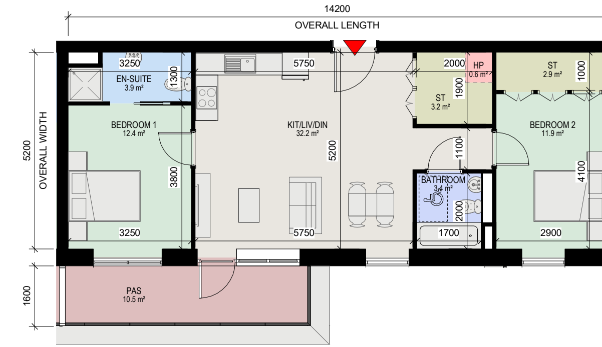
12 Apartment Type 2AJ 1 : 100 - 2 BED, 4 PERSON APARTMENT - GROSS INTERNAL AREA (GIA) : 73.57 sqm
