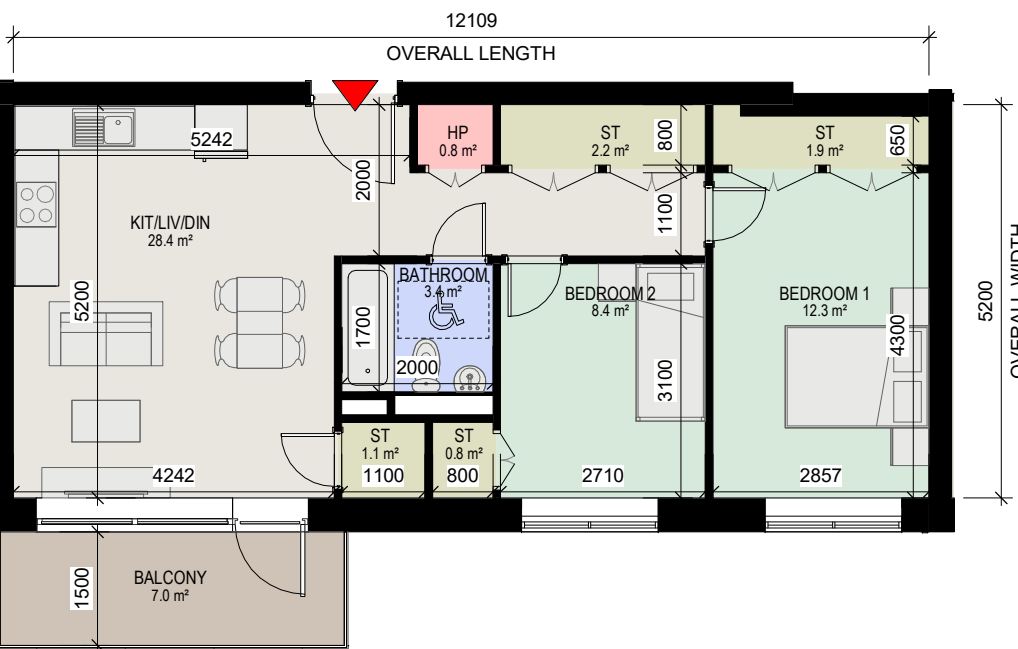
9 Apartment Type 2AG 1 : 100 - 2 BED, 3 PERSON APARTMENT - GROSS INTERNAL AREA (GIA) : 62.59 sqm
