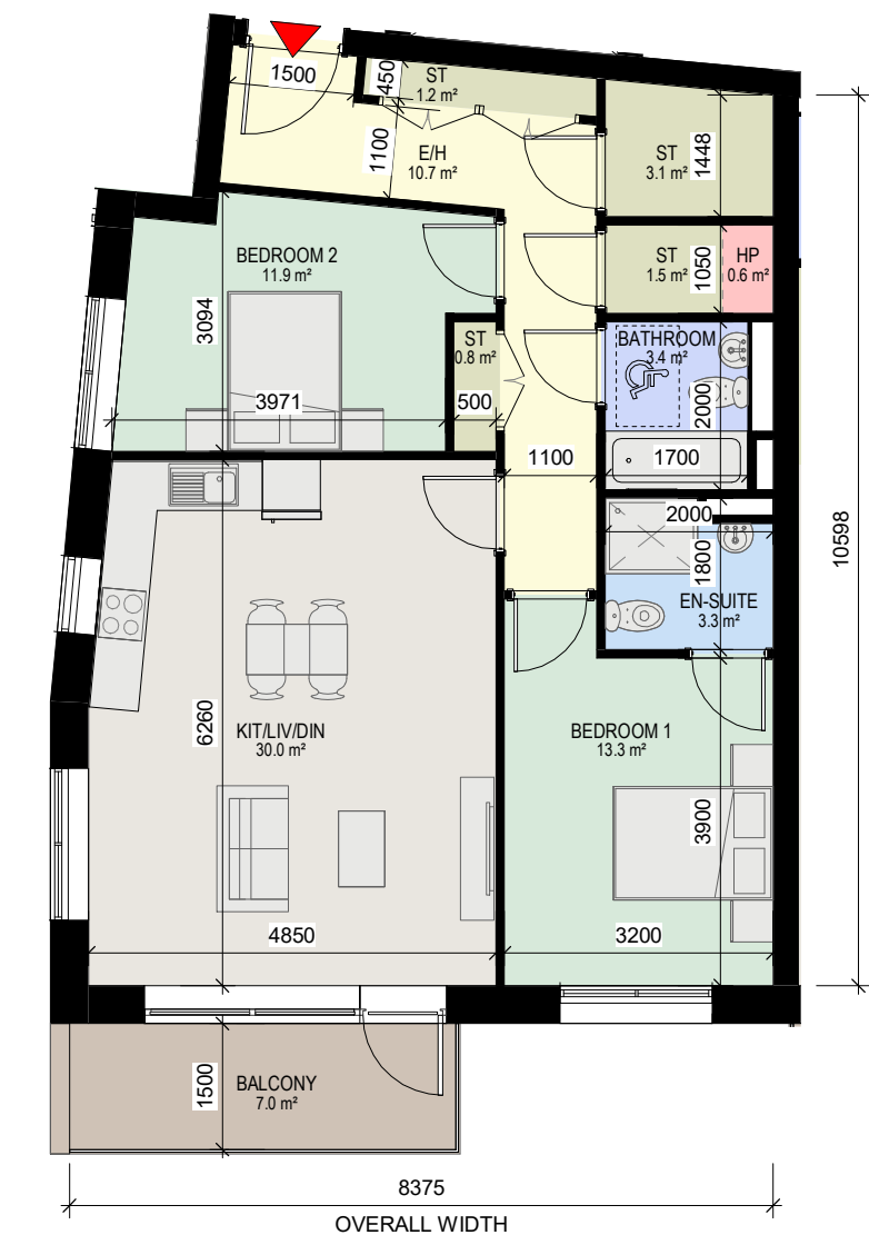
7 Apartment Type 2AE 1 : 100 - 2 BED, 4 PERSON APARTMENT - GROSS INTERNAL AREA (GIA) : 84.41 sqm
