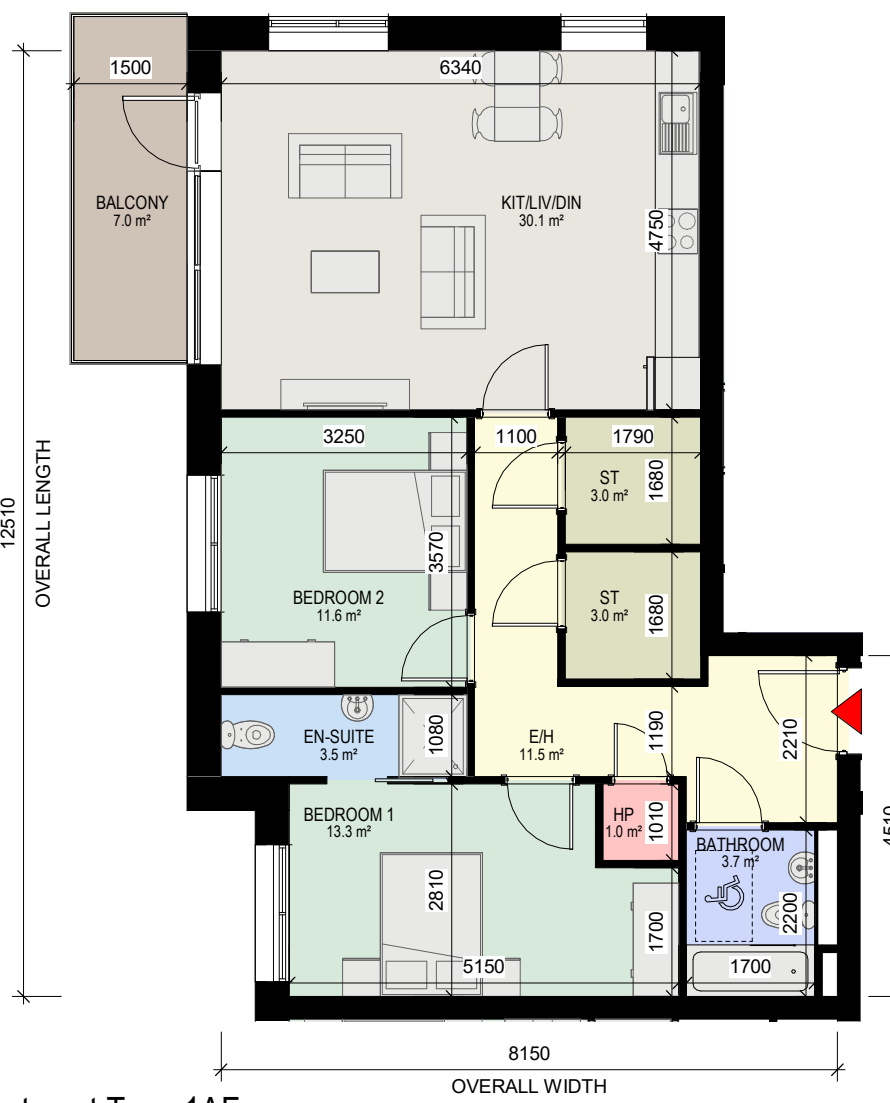
8 Apartment Type 1AF 1 : 100 - 2 BED, 4 PERSON APARTMENT - GROSS INTERNAL AREA (GIA) : 84.86 sqm
