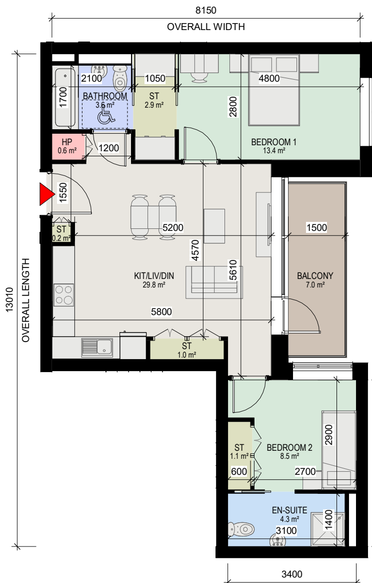
7 Apartment Type 2AE 1 : 100 - 2 BED, 4 PERSON APARTMENT - GROSS INTERNAL AREA (GIA) : 84.41 sqm
