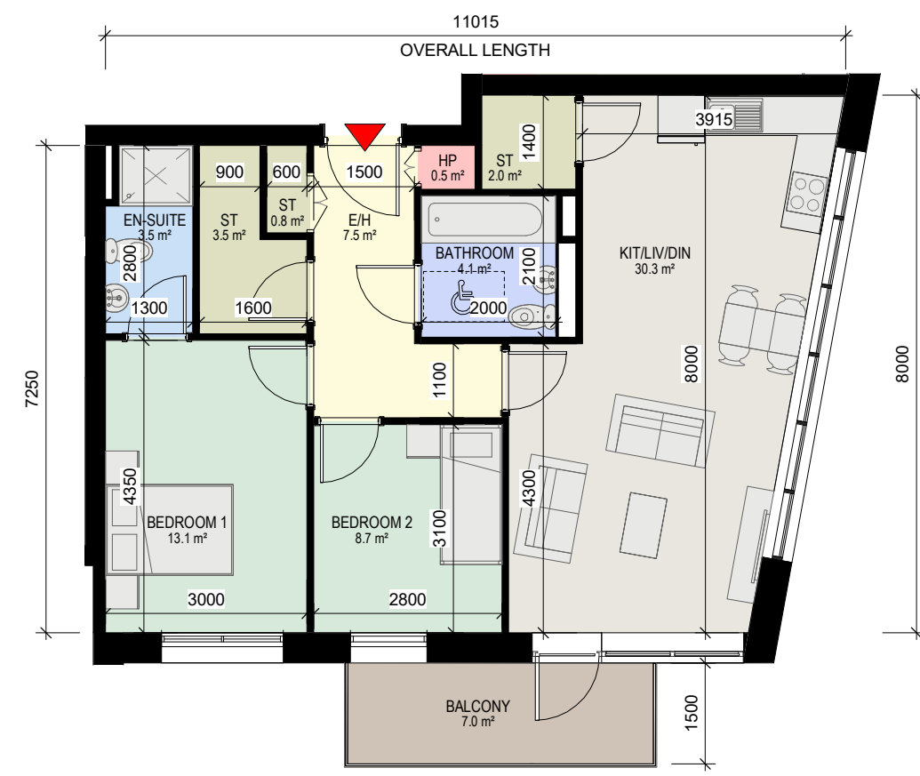
3 Apartment Type 2AA 1 : 100 - 2 BED, 3 PERSON APARTMENT - GROSS INTERNAL AREA (GIA) : 78.13 sqm
