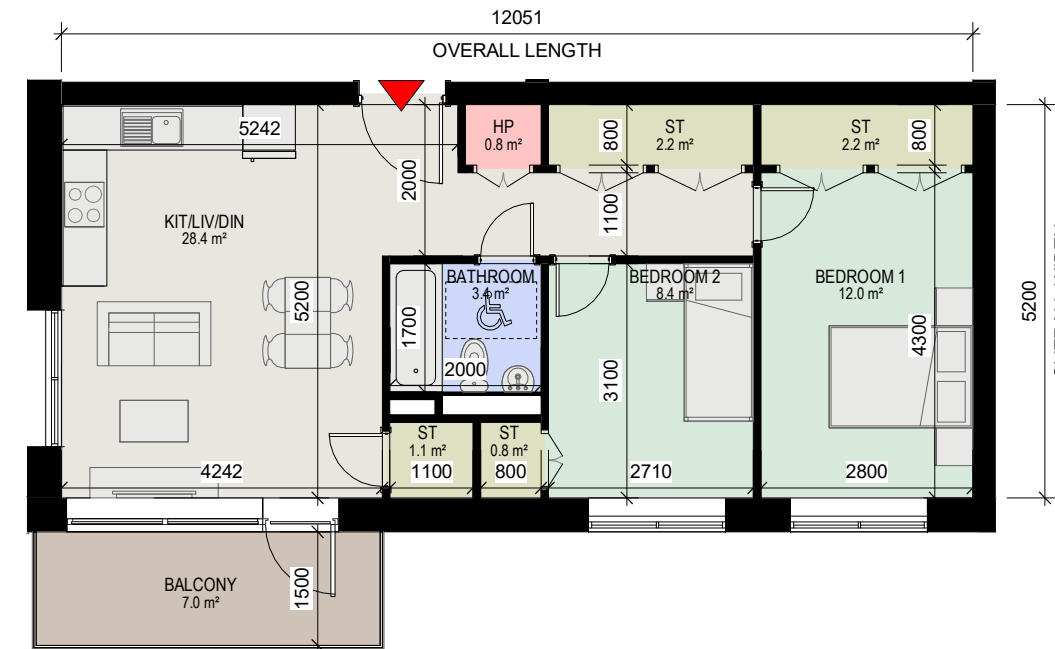
10 Apartment Type 2AH 1 : 100 - 2 BED, 3 PERSON APARTMENT - GROSS INTERNAL AREA (GIA) : 62.66 sqm
