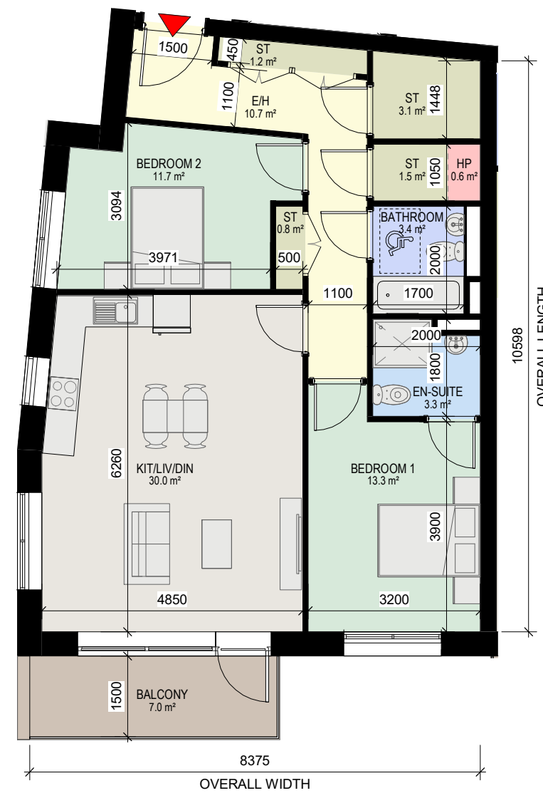
6 Apartment Type 2AD 1 : 100 - 2 BED, 4 PERSON APARTMENT - GROSS INTERNAL AREA (GIA) : 84.26 sqm
