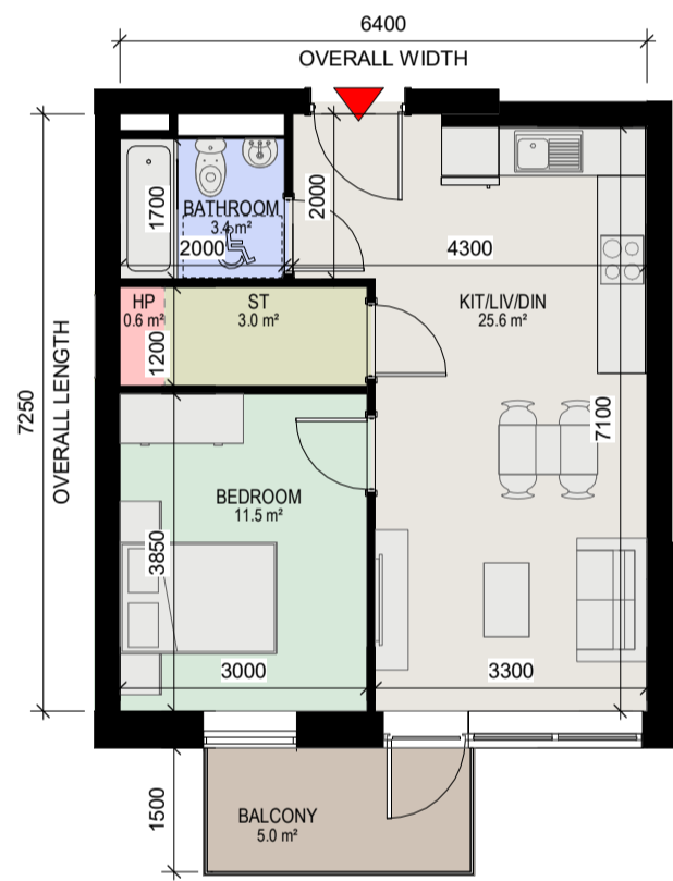
7 Apartment Type 1V 1 : 100
