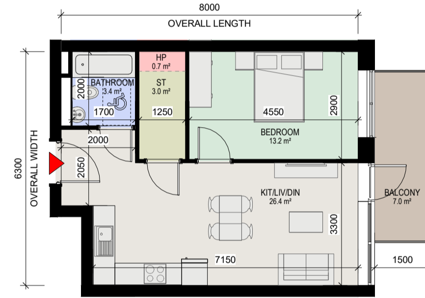
8 Apartment Type 1W 1 : 100
