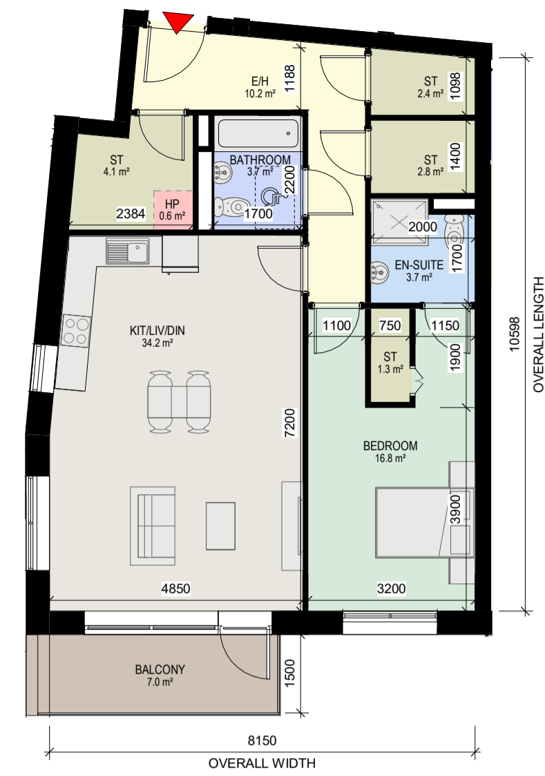
4 Apartment Type 1S 1 : 100
