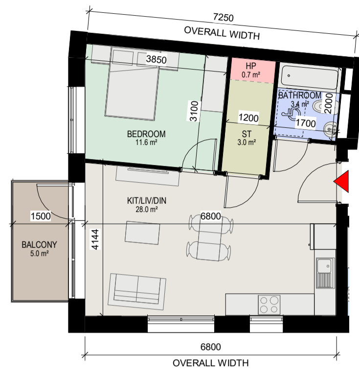
1 Apartment Type 1P 1 : 100
