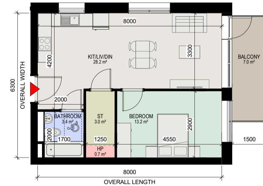
9 Apartment Type 1X 1 : 100
