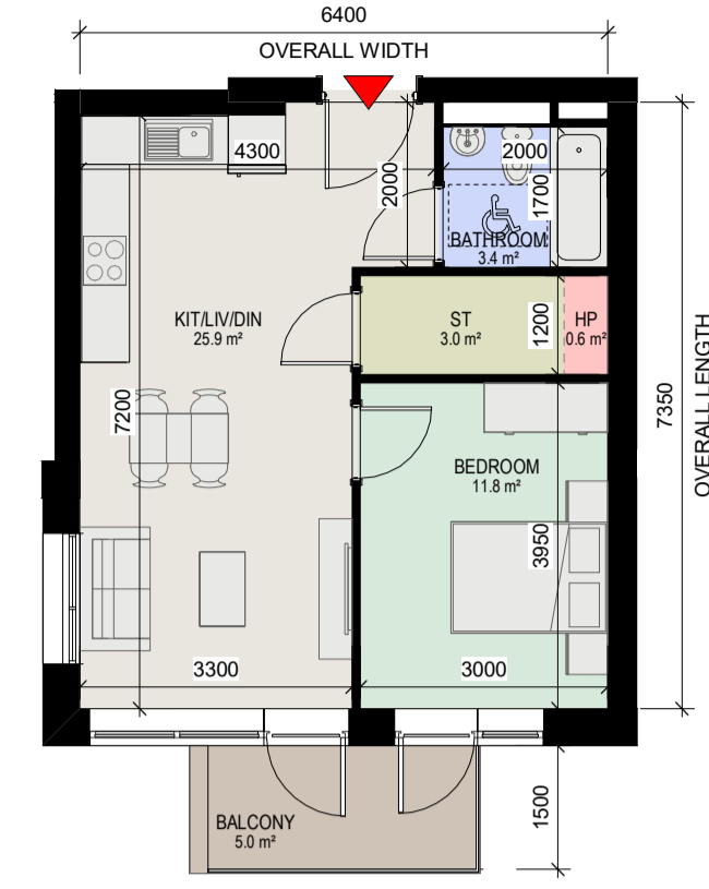
5 Apartment Type 1T 1 : 100
