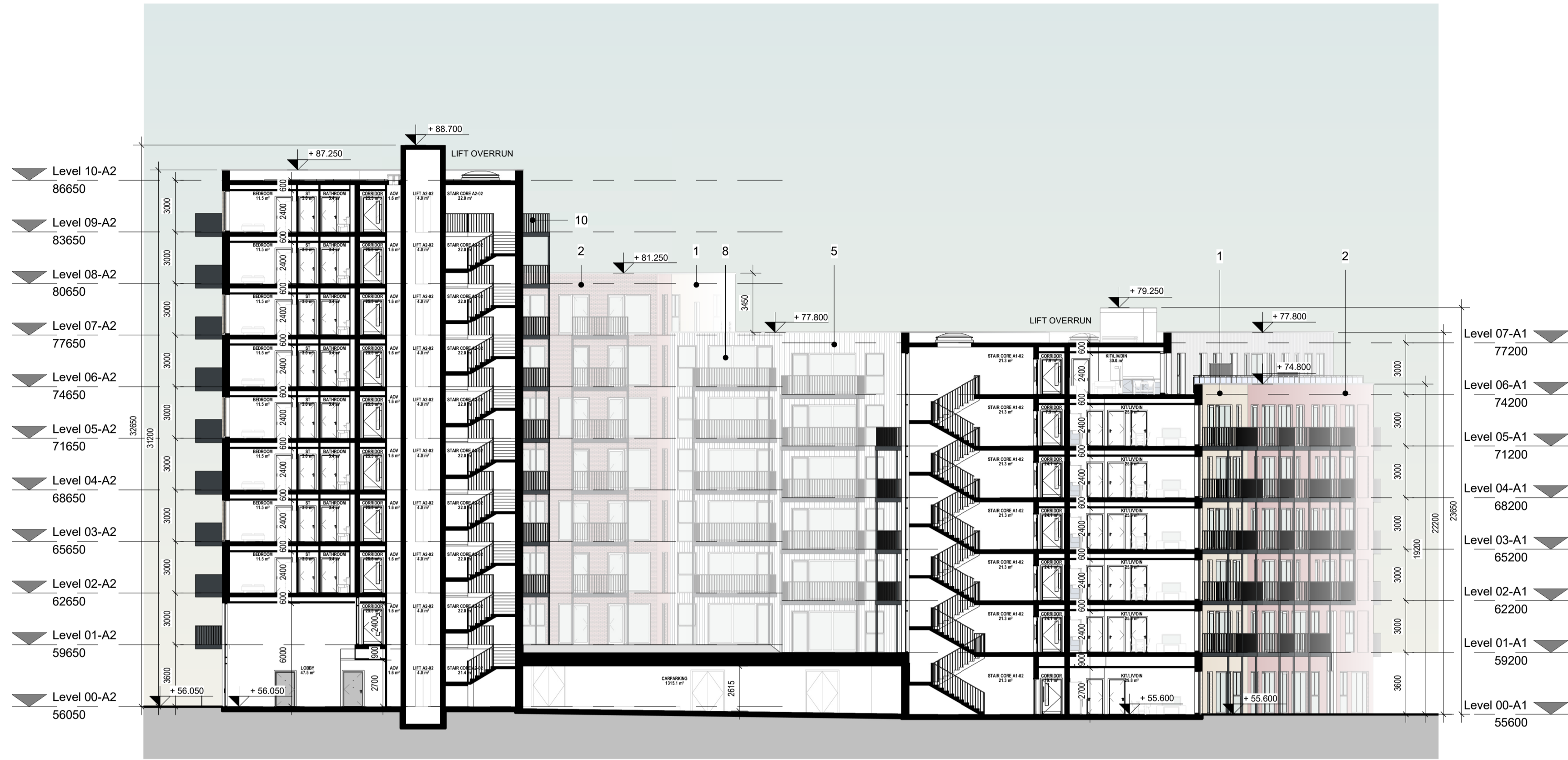
1 BLOCK A-SECTION C-C 1 : 200
