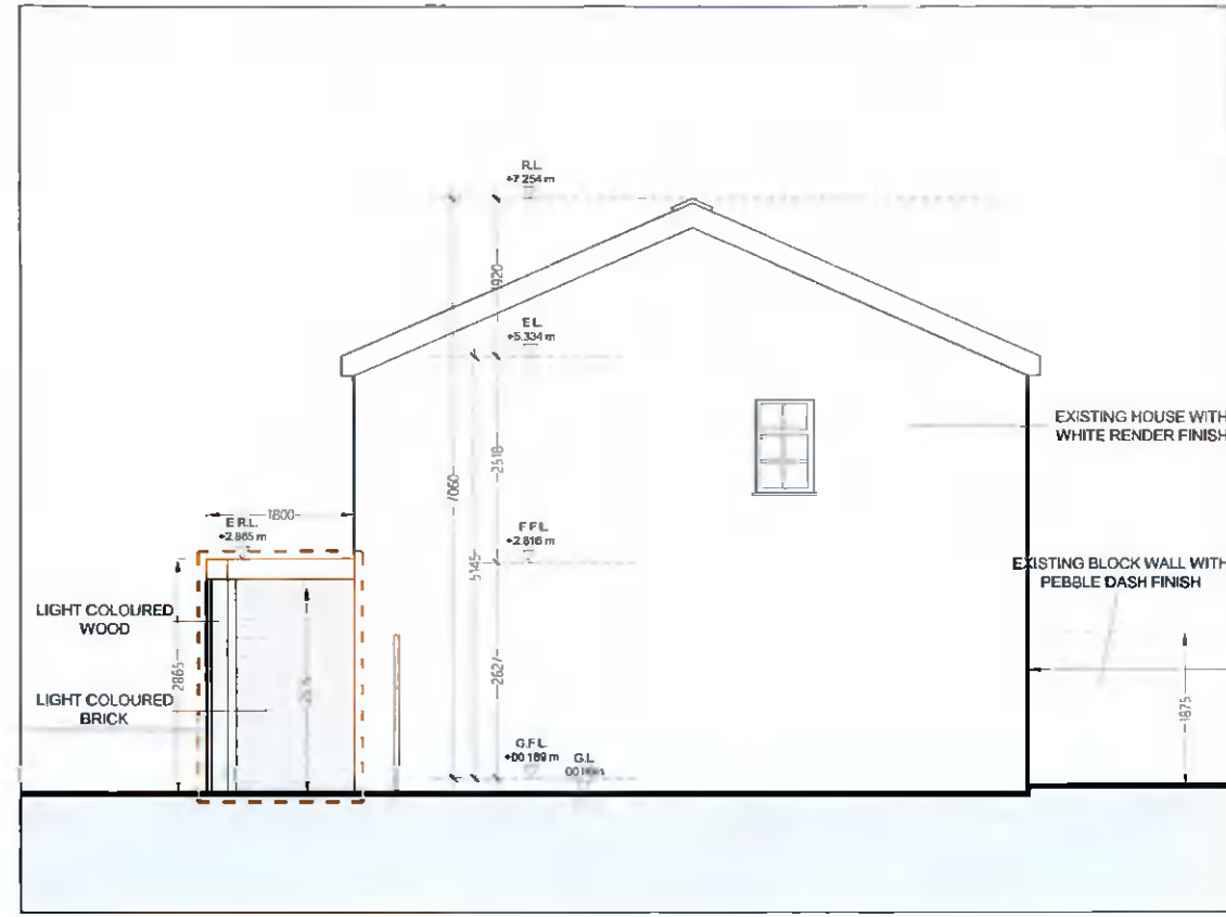
2 - SIDE ELEVATION (WEST)
