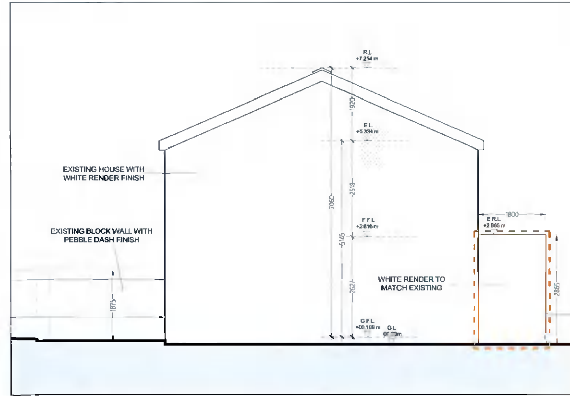
4 - SIDE ELEVATION (EAST)
