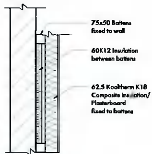
DRY LINING DETAIL Scale 1:20
