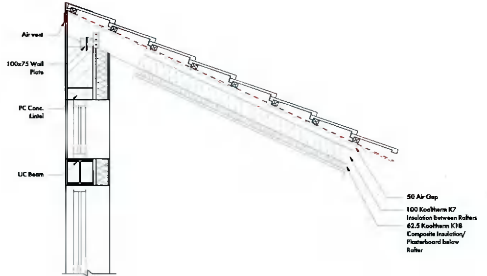
DETAIL 2 Scale 1:20
