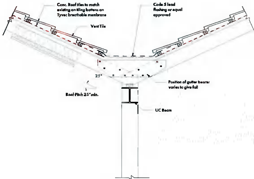
DETAIL 1 Scale 1:20
