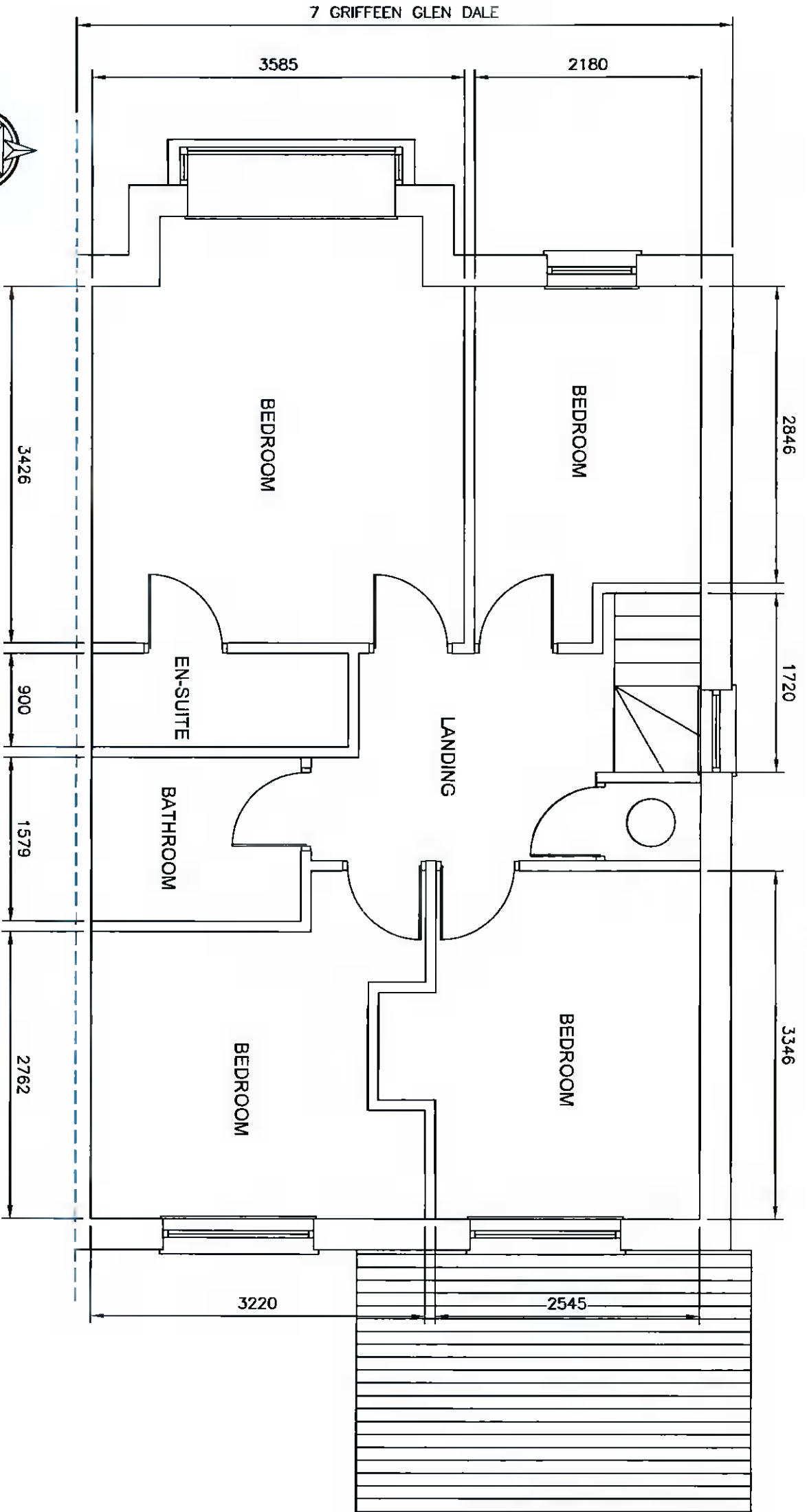
EXISTING FIRST FLOOR PLAN VIEW
