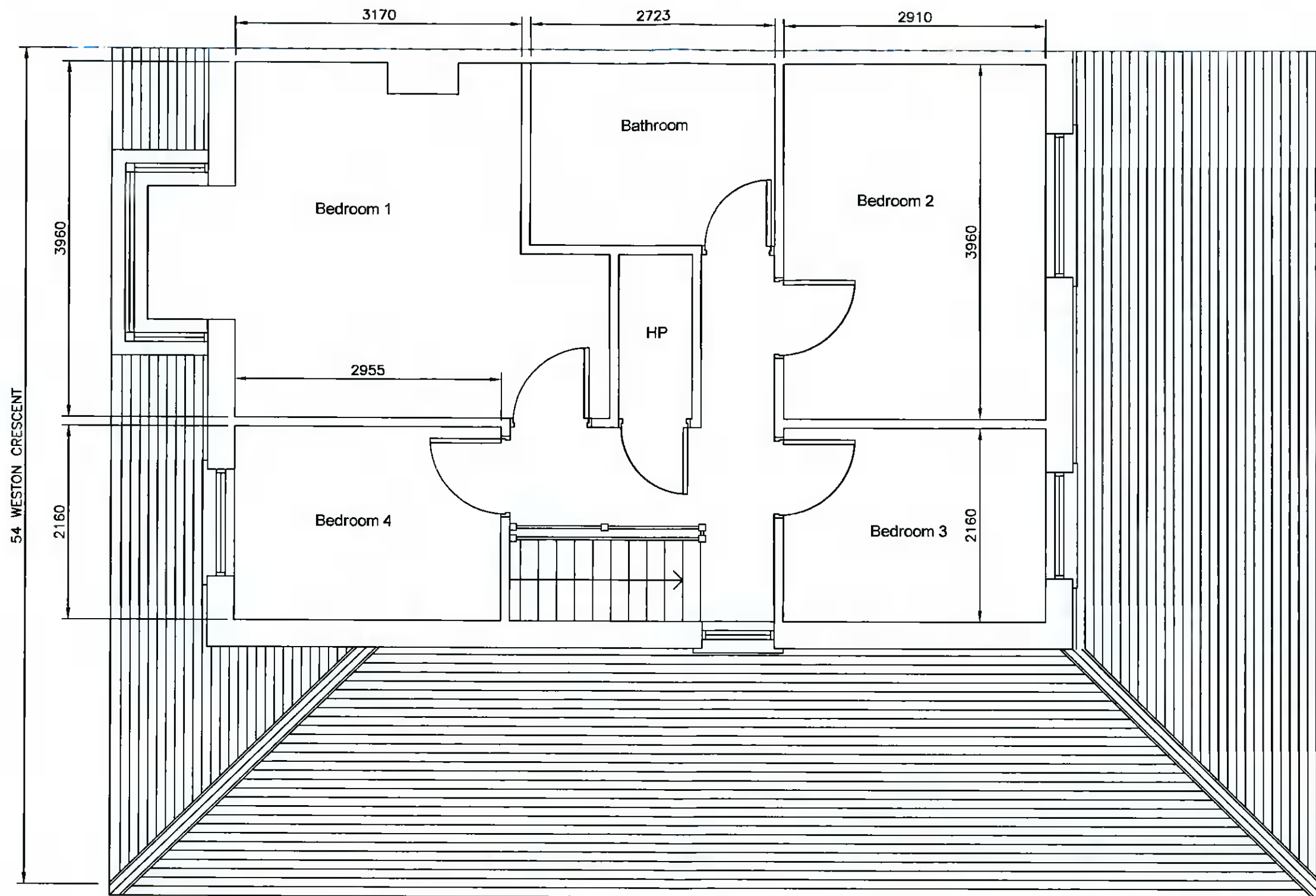
EXISTING FIRST FLOOR PLAN VIEW
