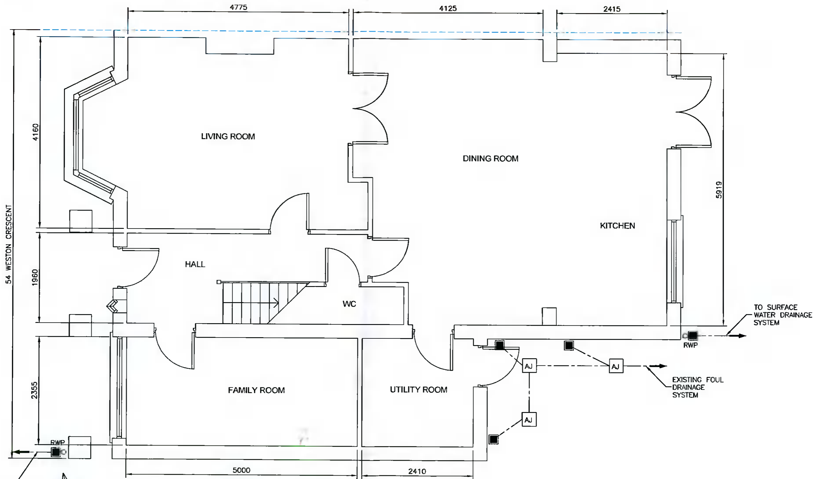
EXISTING GROUND FLOOR PLAN VIEW
