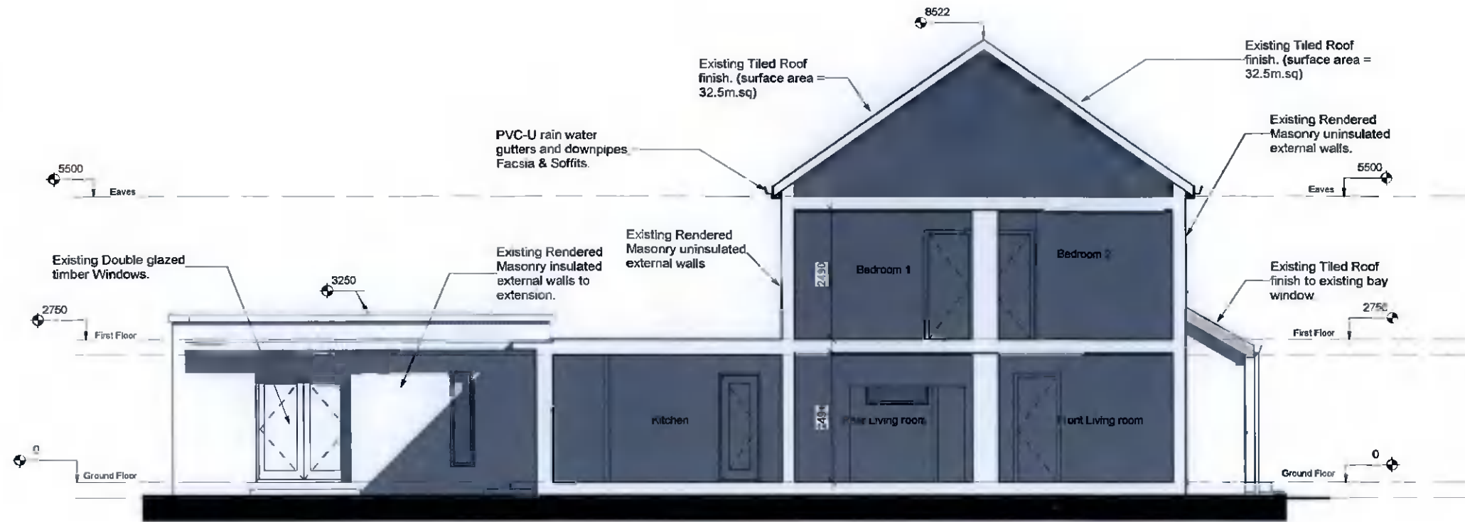
SECTION 1 (SHOWING WEST ELEVATION) - 1:100@A3
