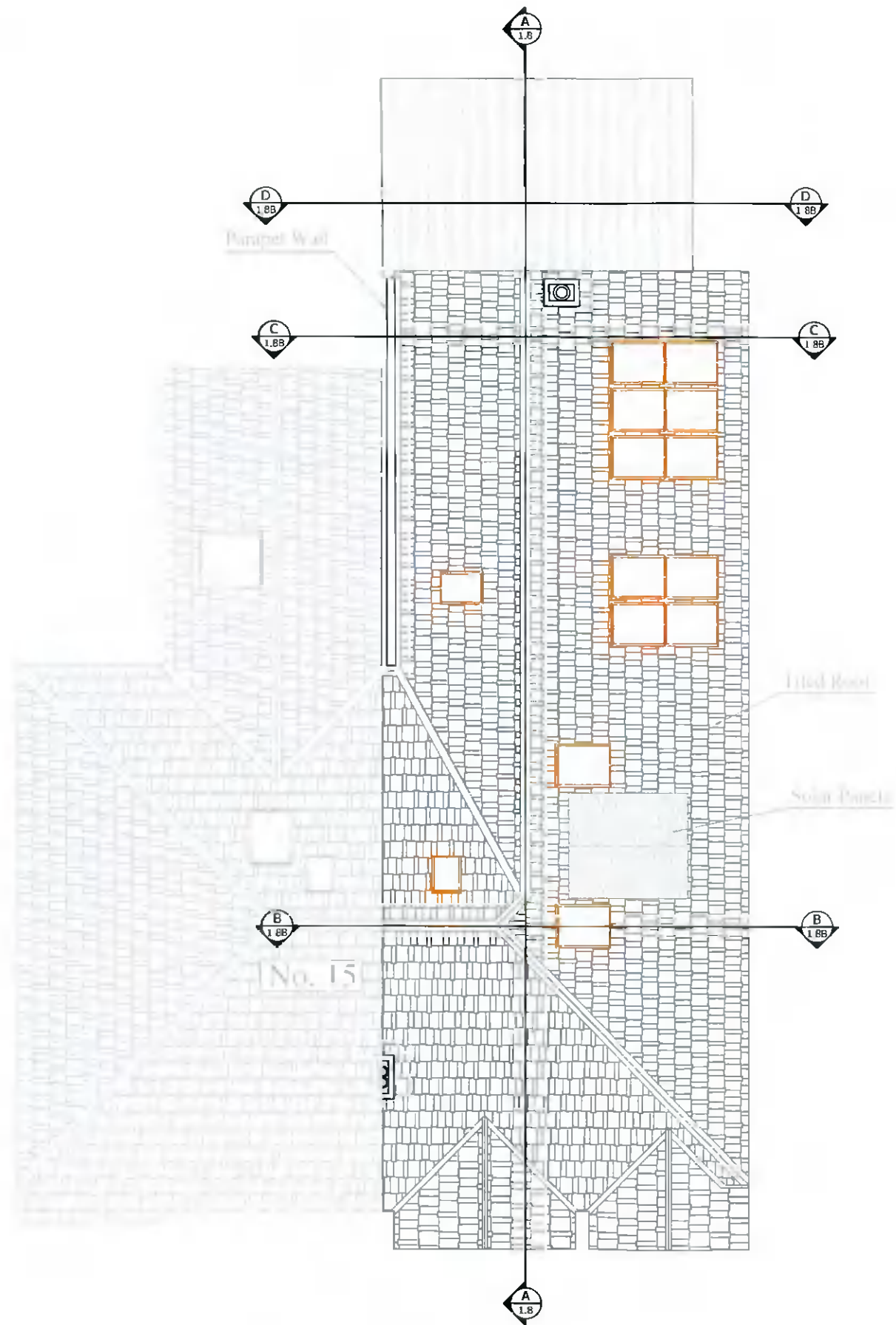
5 Existing Roof Plan Scale: 1:100
