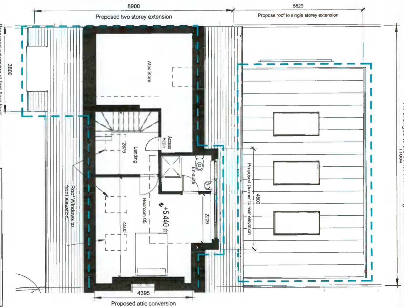
Proposed -3-Second Floor 1 : 100
