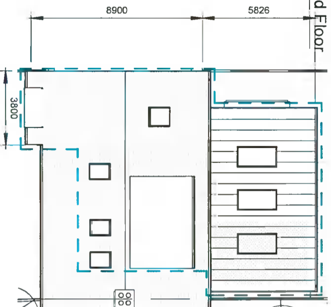
Proposed -4-Roof Plan 1 : 200
