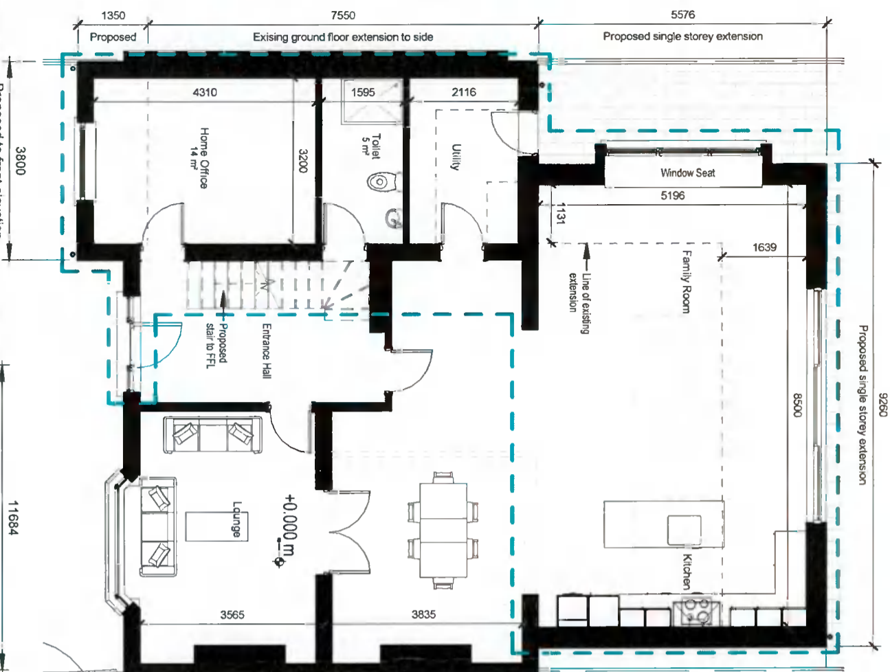
Proposed -1-Ground Floor 1 : 100
