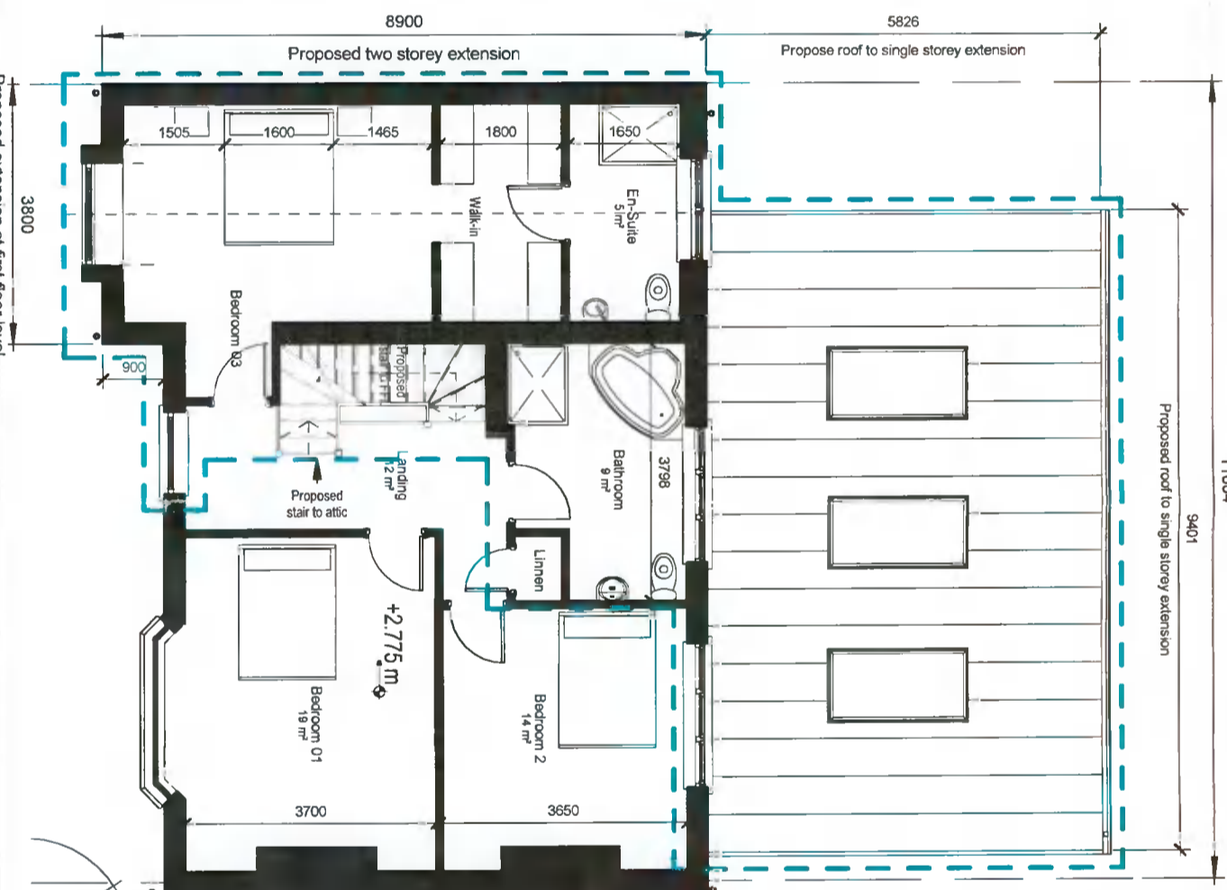
Proposed -2-First Floor 1 : 100
