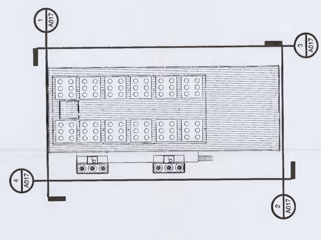
MULTIFUEL POWER PLANT NORTH BUILDING - KEY PLAN 1:500
