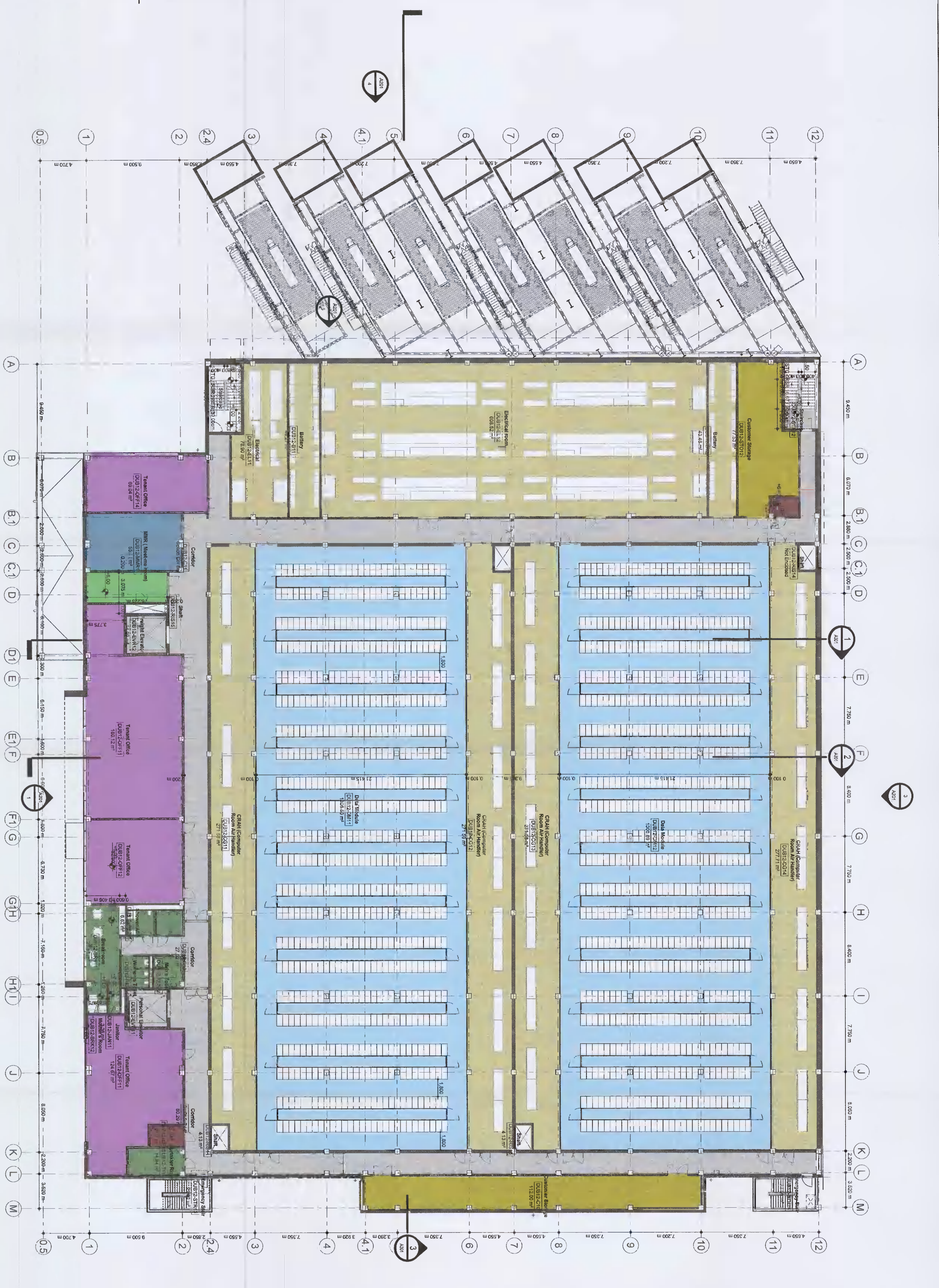
1 DUB12 OVERALL FIRST FLOOR PLAN SCALE: 1:300
