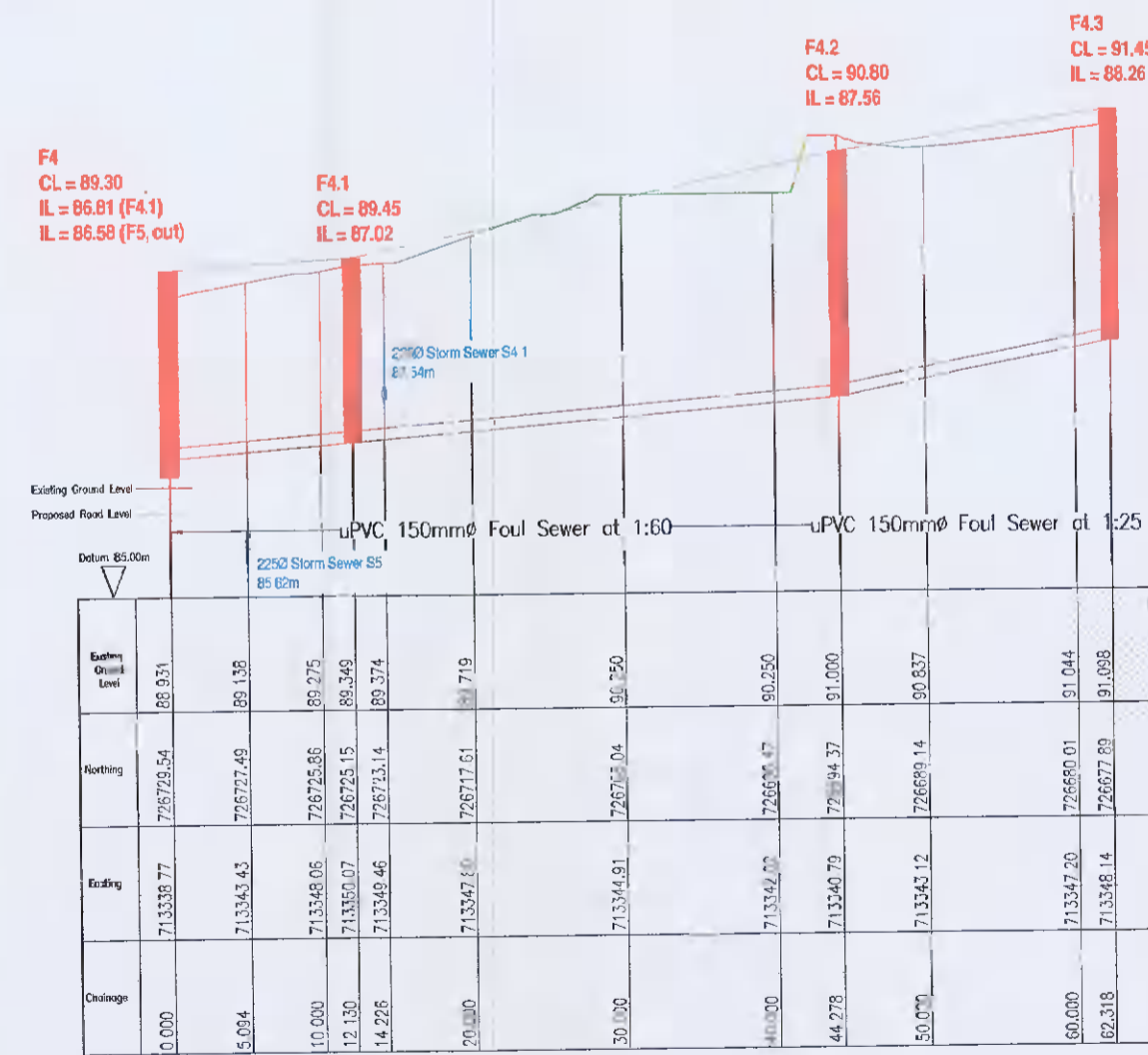
FOUL SEWER F4 TO F4.3 LONGITUDINAL SECTION Scale 1:500 Horizontal, 1:100 Vertical
