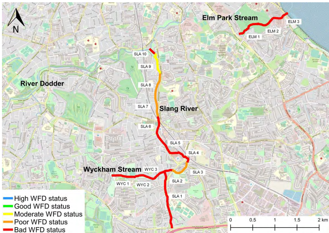
Figure 4.16 RHAT scores (equivalent to WFD status) along the Wyckham Stream, Slang River and Elm Park Stream surveyed in Dublin City boundaries, April 2018-April 2019
