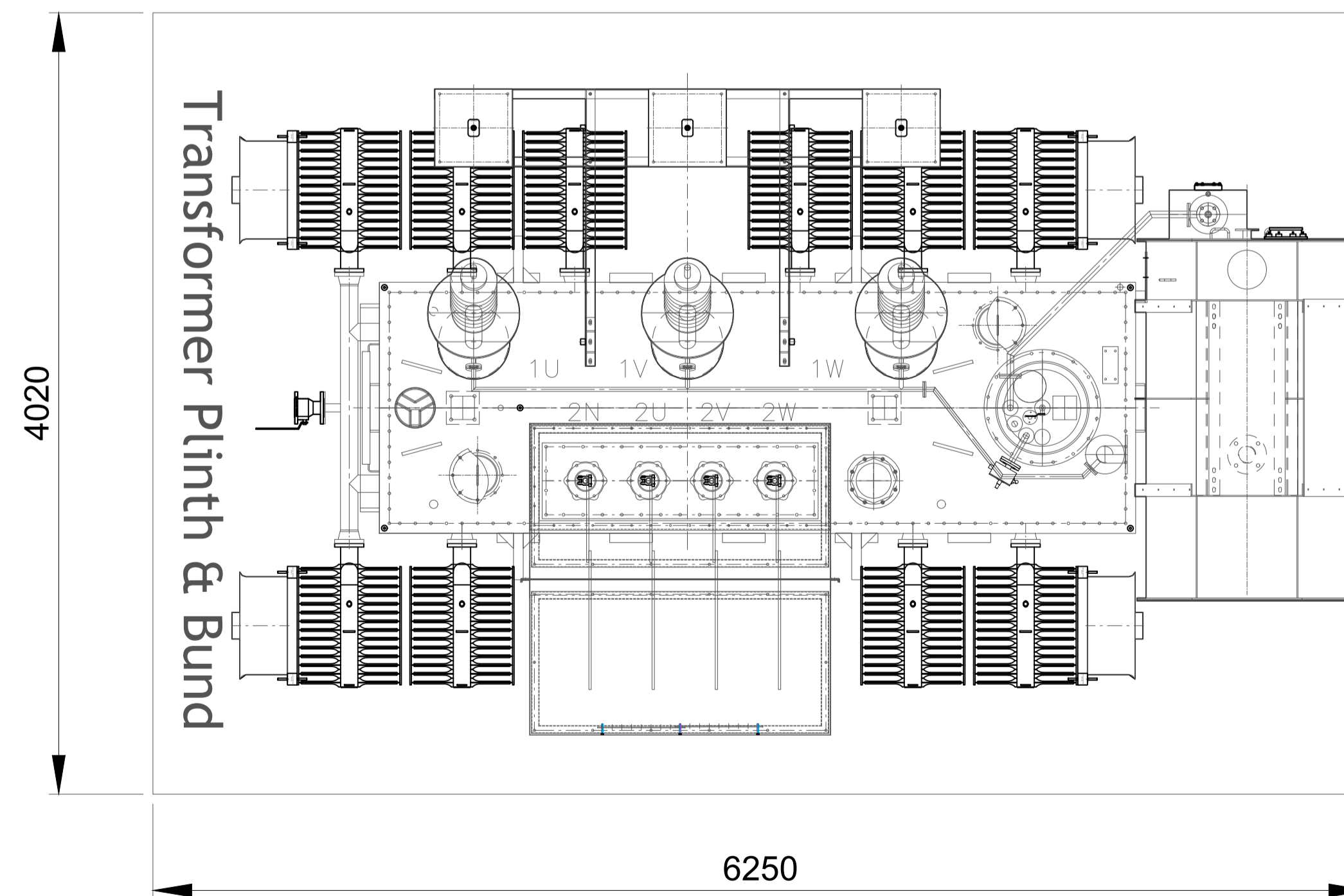
PLAN
