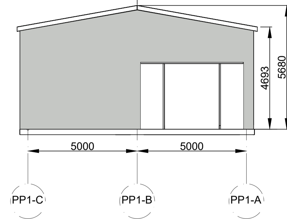
Elevation S1
