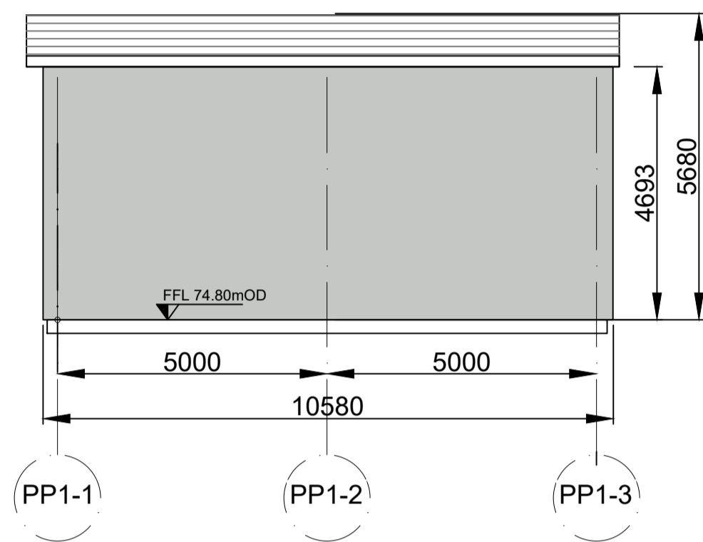
Elevation S2
