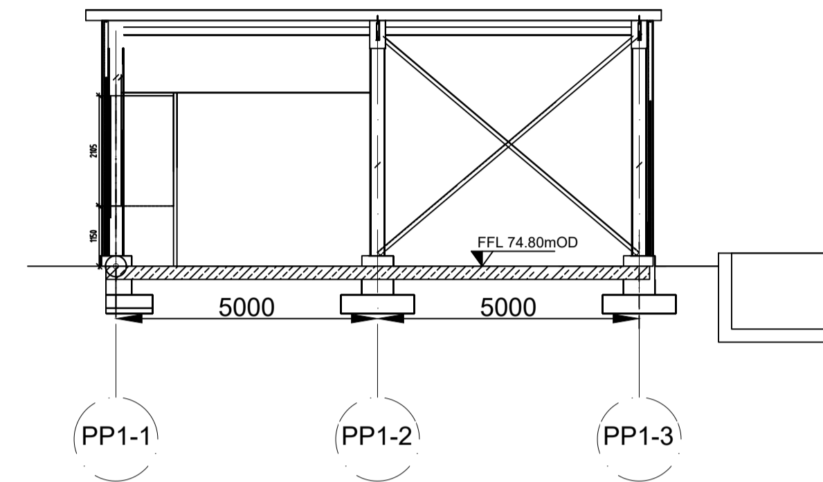
Section S2 (1:125)
