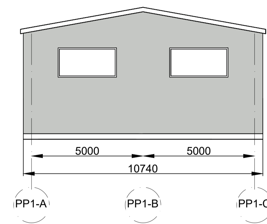
Elevation S3
