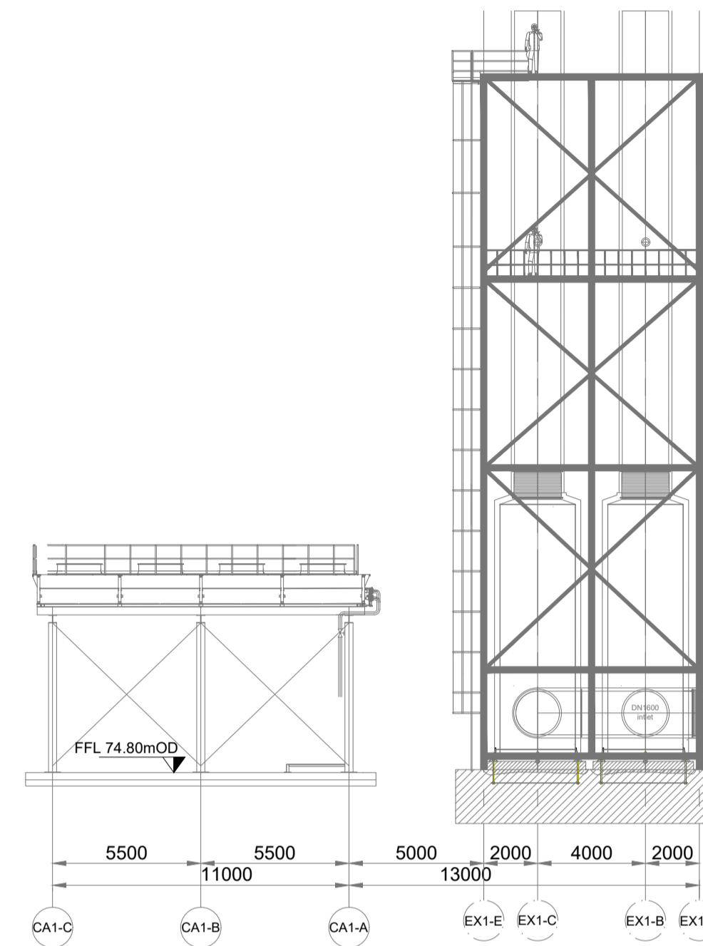
SECTION 1-1 Scale 1:200
