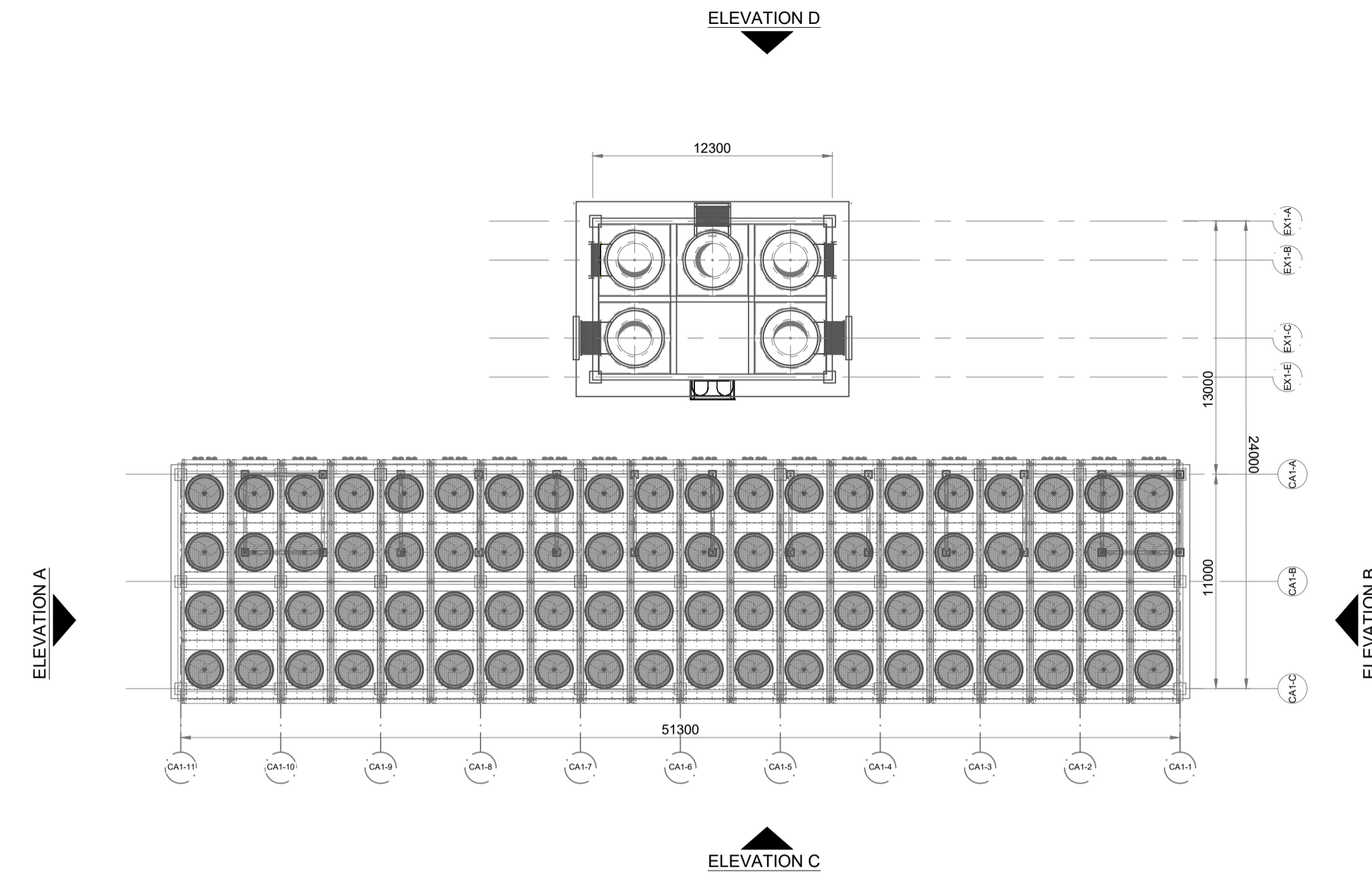
PLAN Scale 1:250
