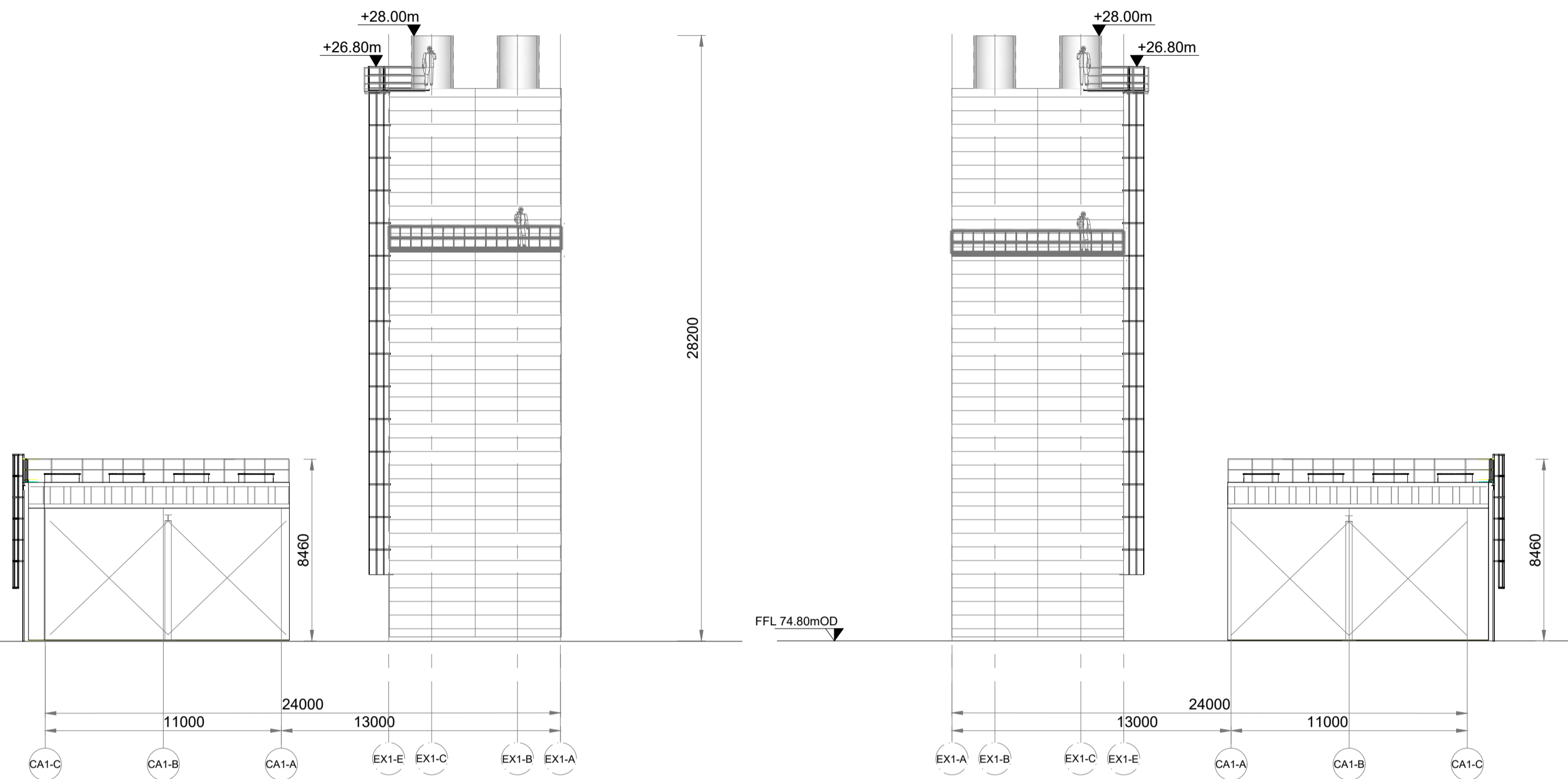
ELEVATION A Scale 1:200
