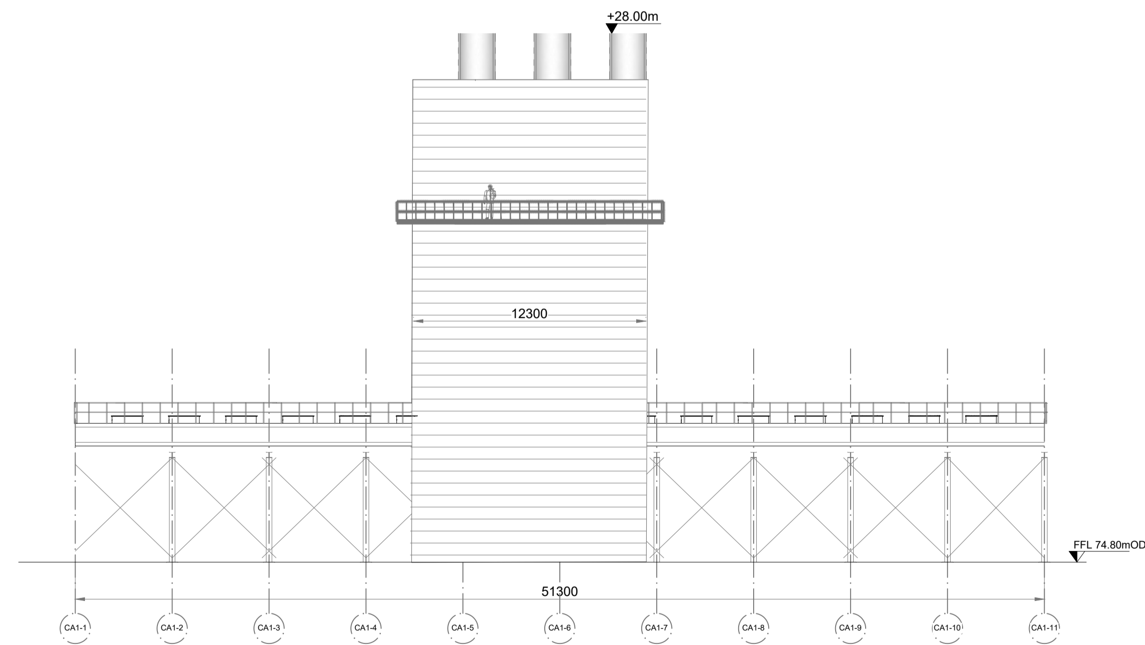
ELEVATION D Scale 1:200
