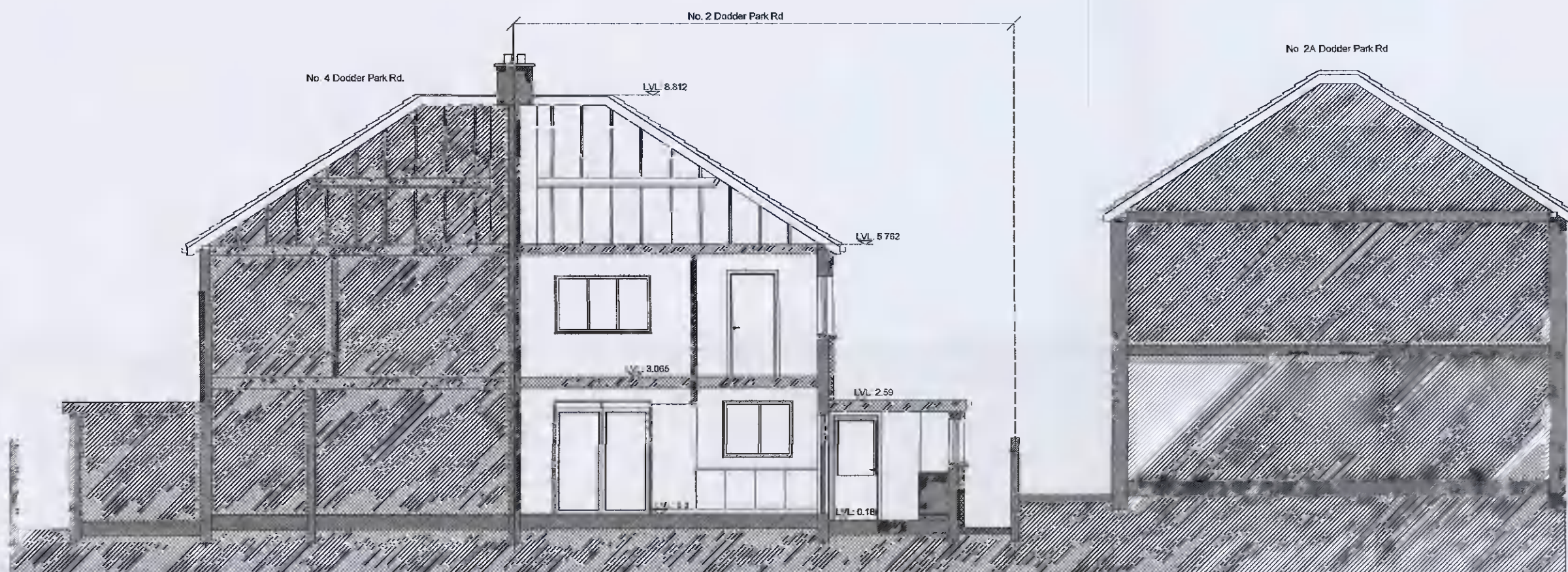
Section E-E
