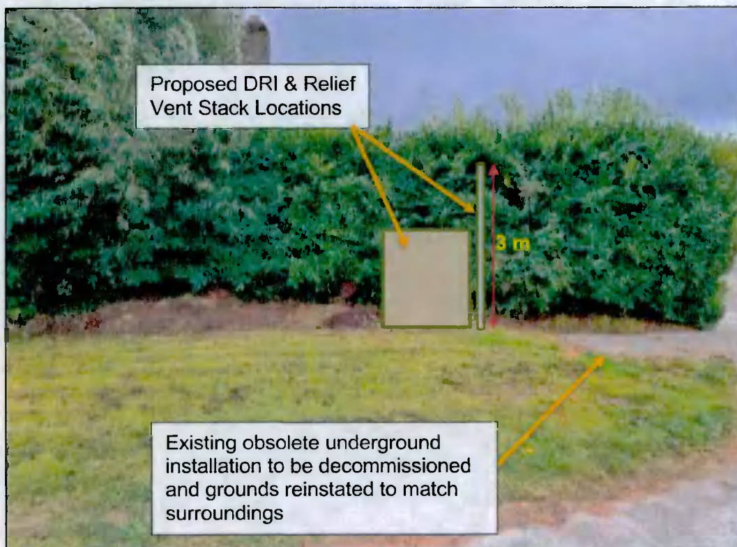
Figure 2 - Proposed DRI & Relief Vent Stack Locations
