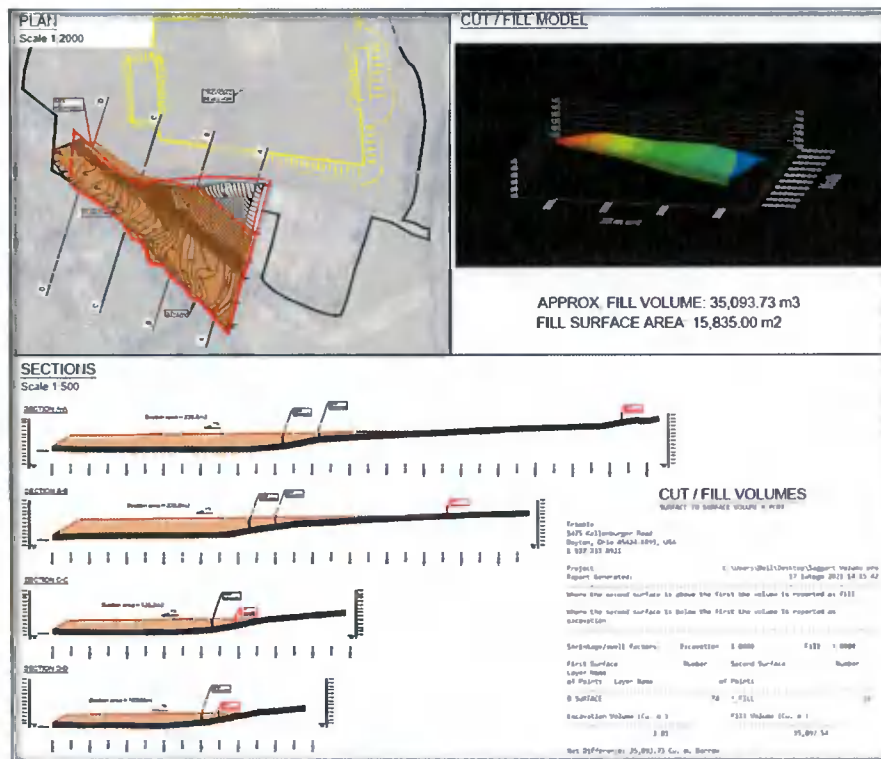
Figure 2 – An Extract from Planning Drawings Submitted
