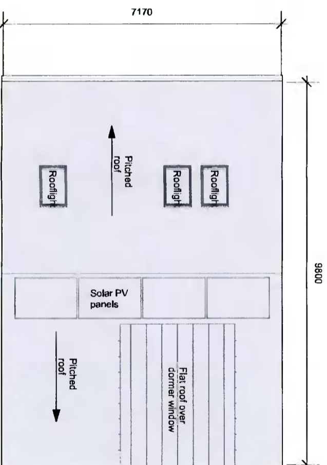
ROOF PLAN
