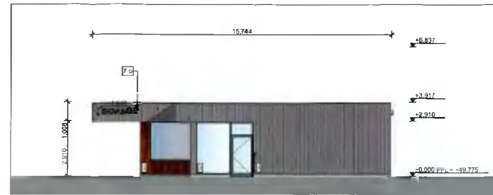
③ Elevation B 1:200
