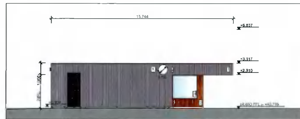
⑤ Elevation D 1:200
