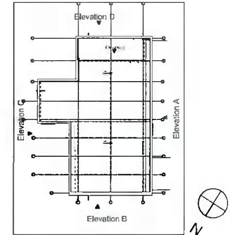
① KEY PLAN
