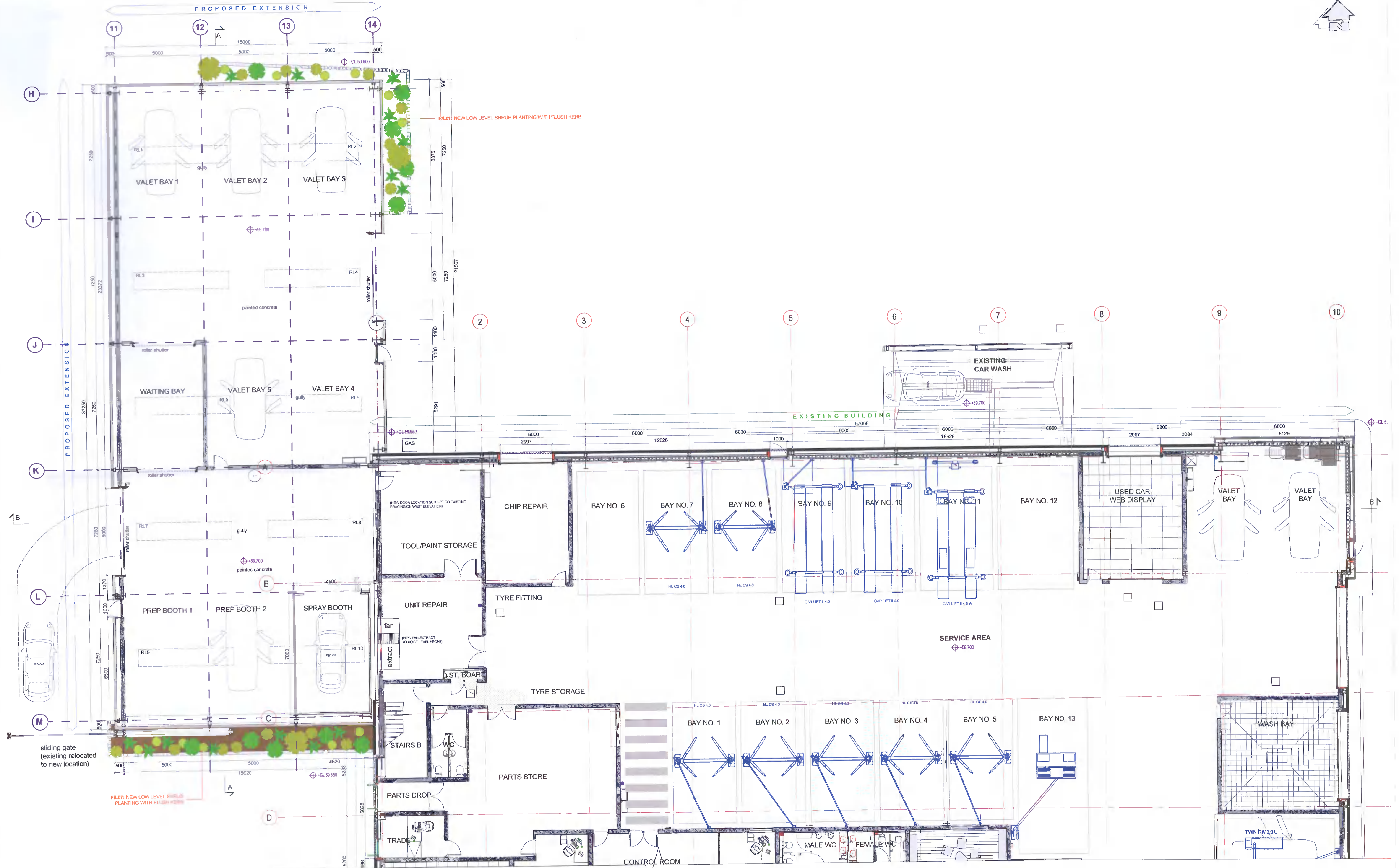
PART EXISTING FLOOR PLAN: REFER TO EXISTING GROUND FLOOR PLAN & PA_3-00 PROPOSED GROUND FLOOR PLAN 1:200
