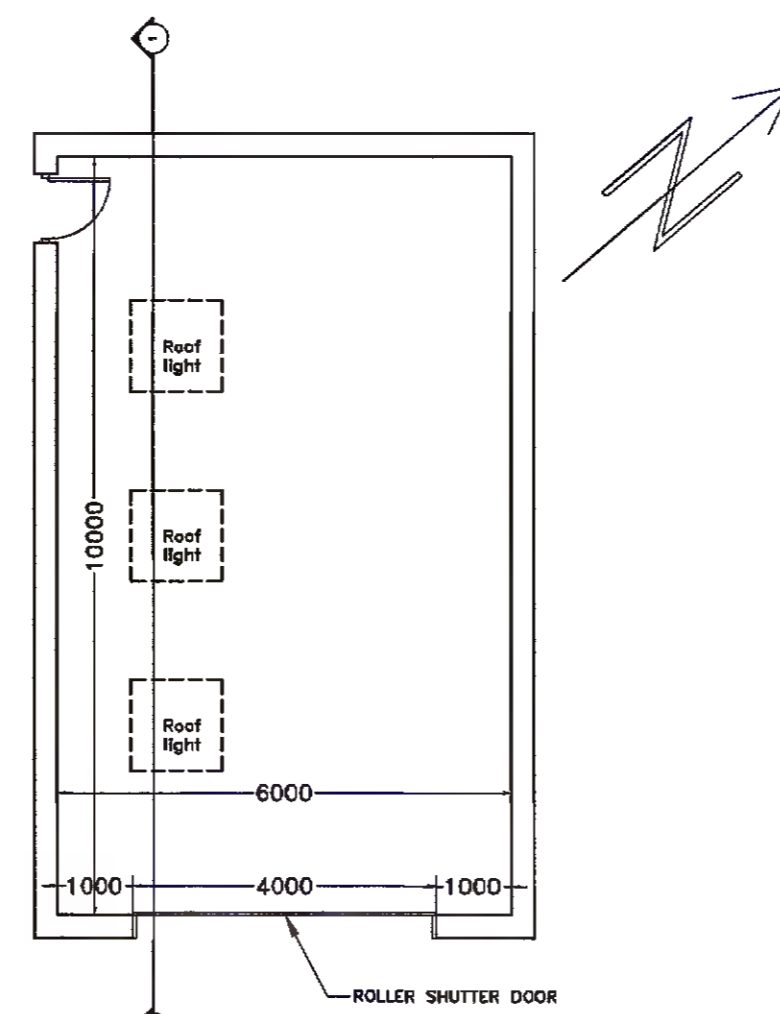
GARAGE (PROPOSED) SCALE 1:100
