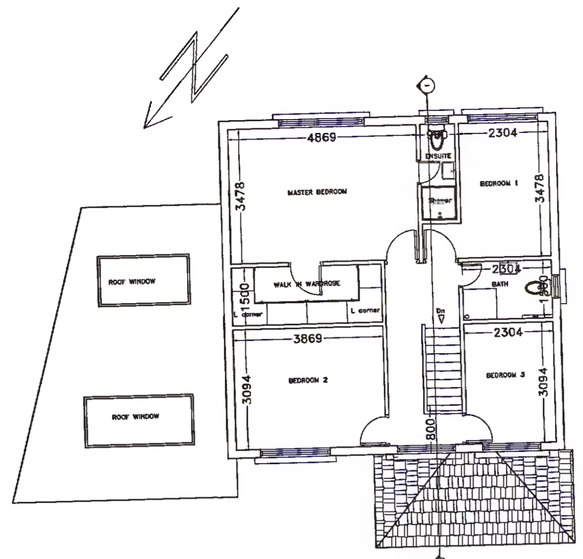
NO.22 FIRST FLOOR LAYOUT (EXISTING) SCALE 1:100
