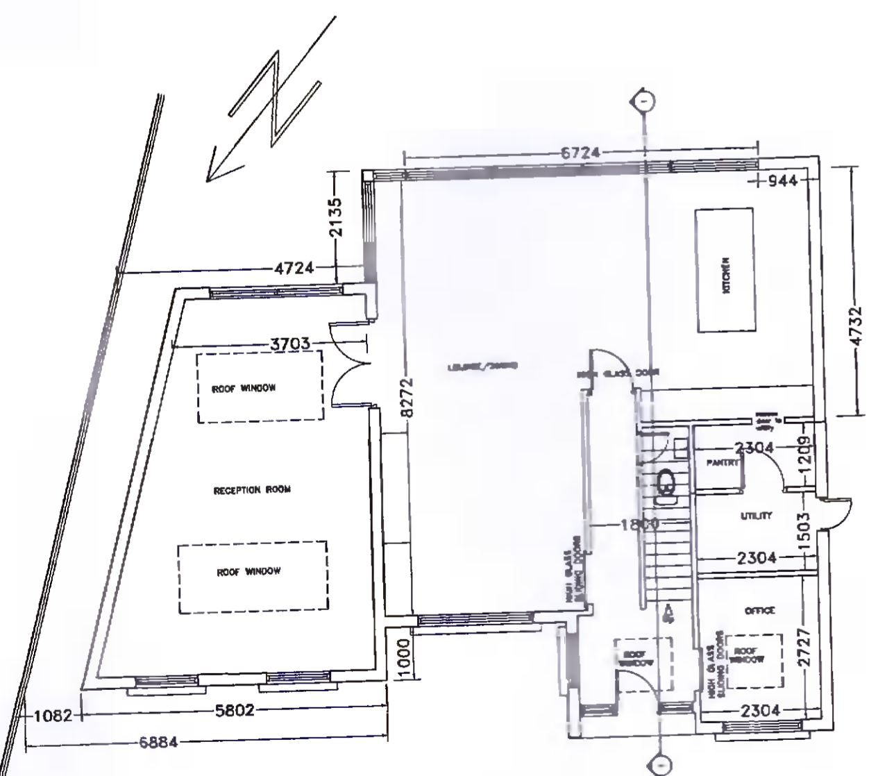
NO.22 GROUND FLOOR LAYOUT (PROPOSED) SCALE 1:100
