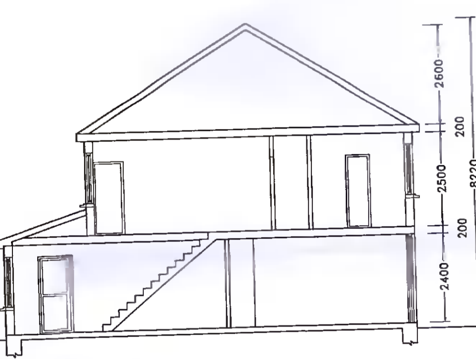
MAIN SECTION (EXISTING) SCALE 1:100
