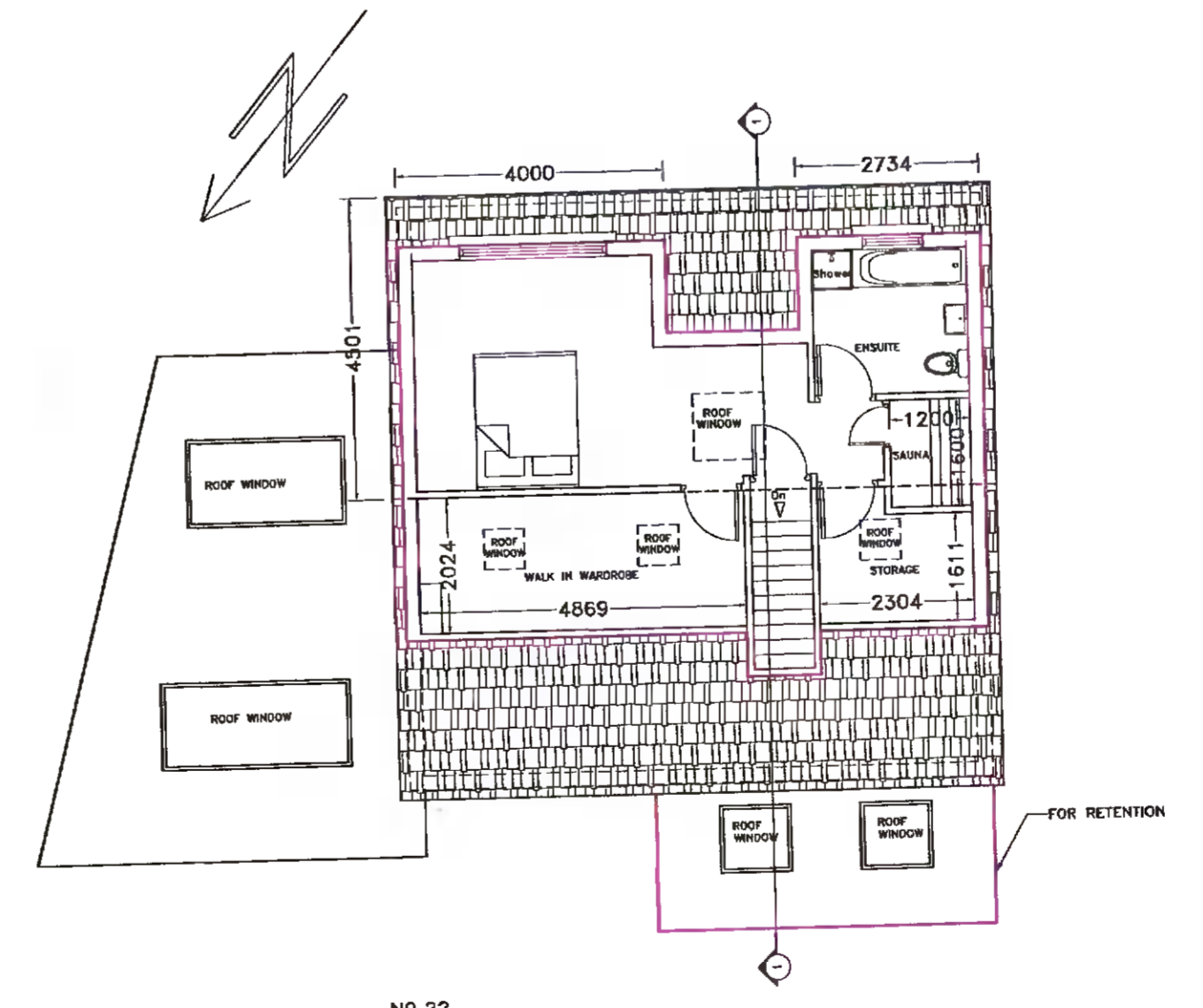
NO.22 ATTIC FLOOR LAYOUT (PROPOSED) SCALE 1:100
