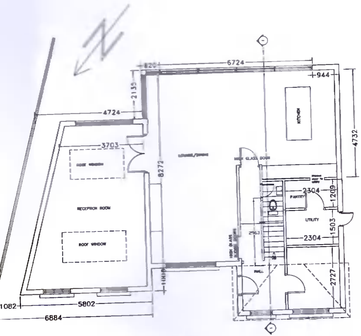
NO.22 GROUND FLOOR LAYOUT (EXISTING) SCALE 1:100
