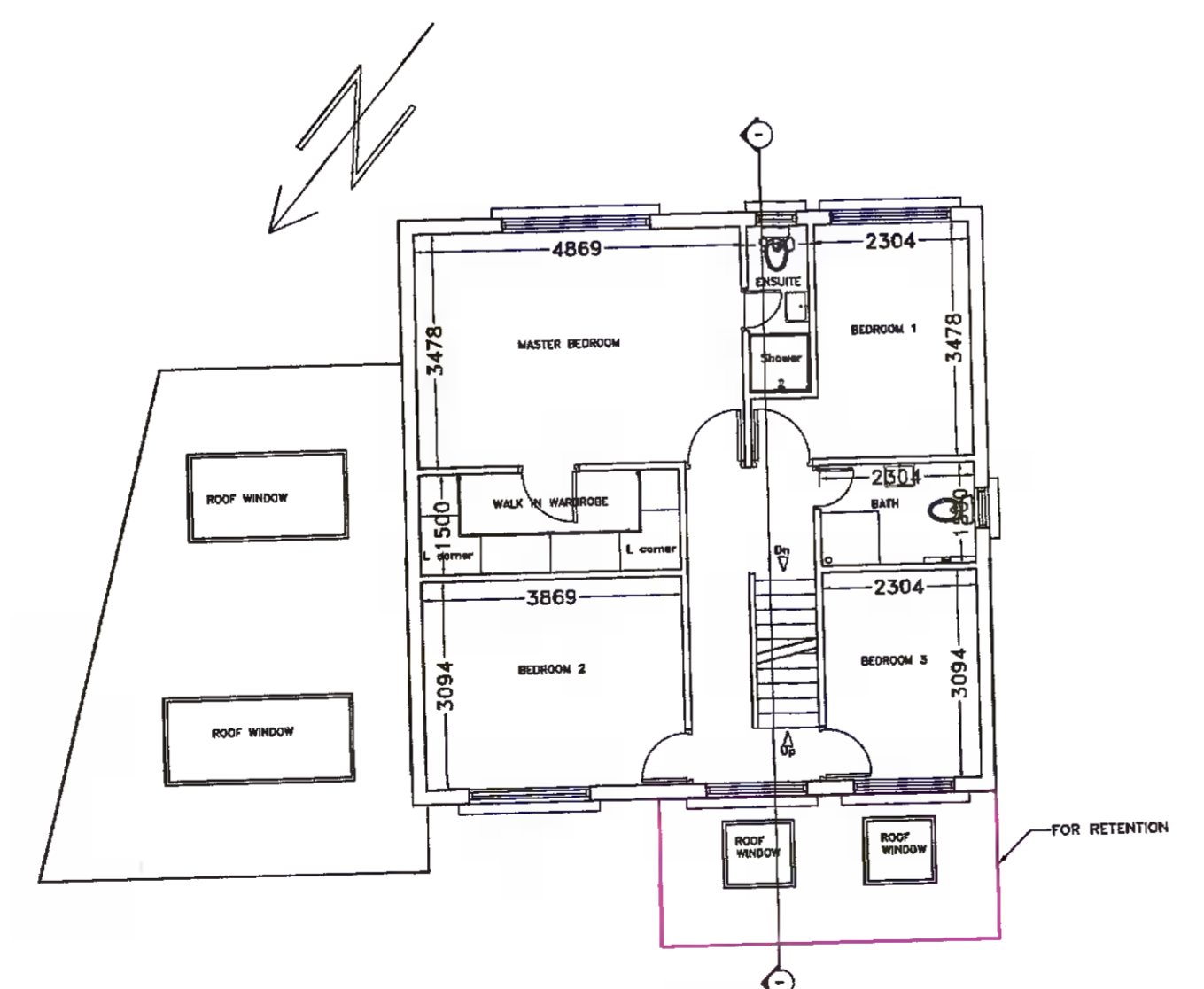
NO.22 FIRST FLOOR LAYOUT (PROPOSED) SCALE 1:100
