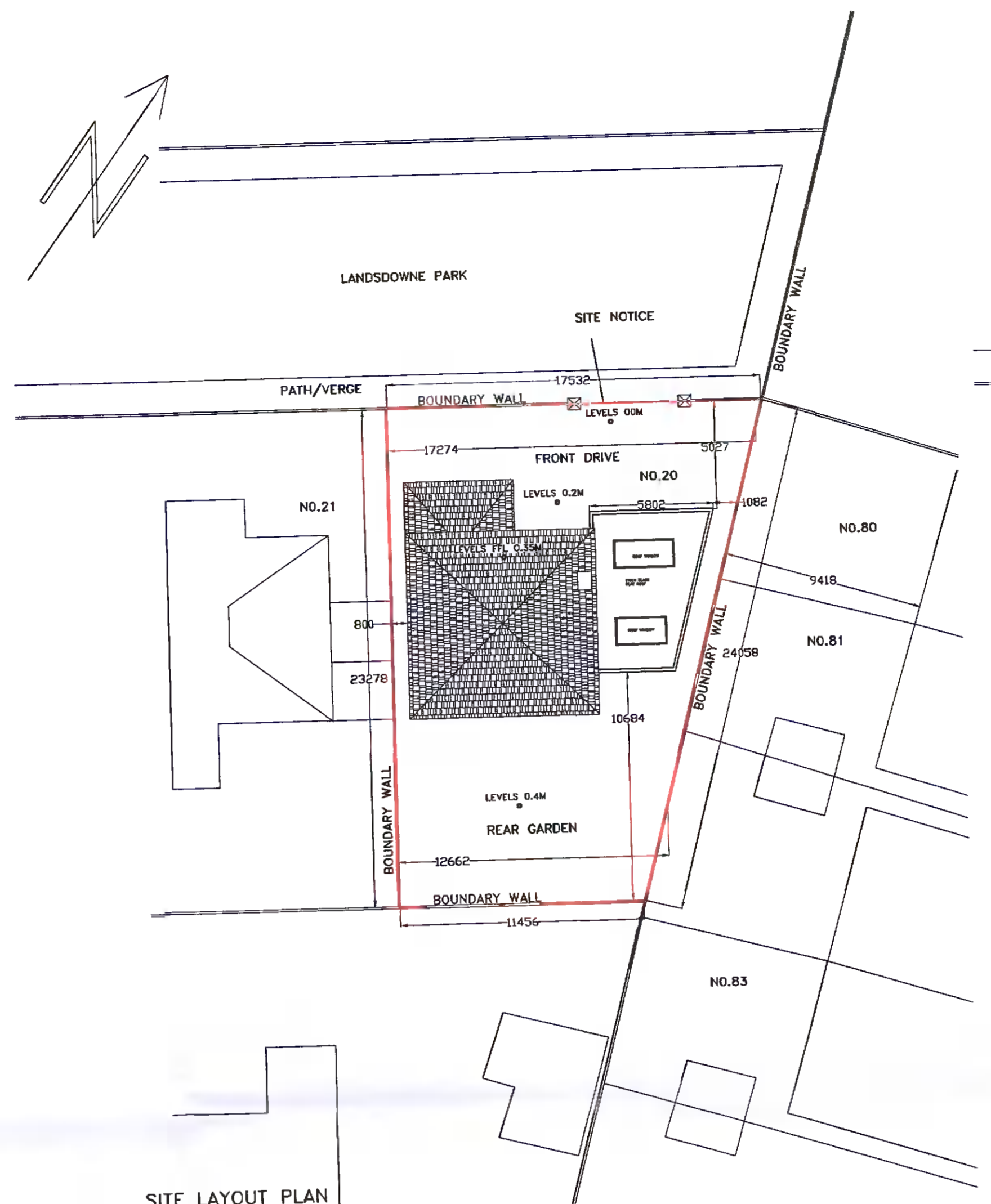
SITE LAYOUT PLAN (EXISTING) SCALE 1:200
