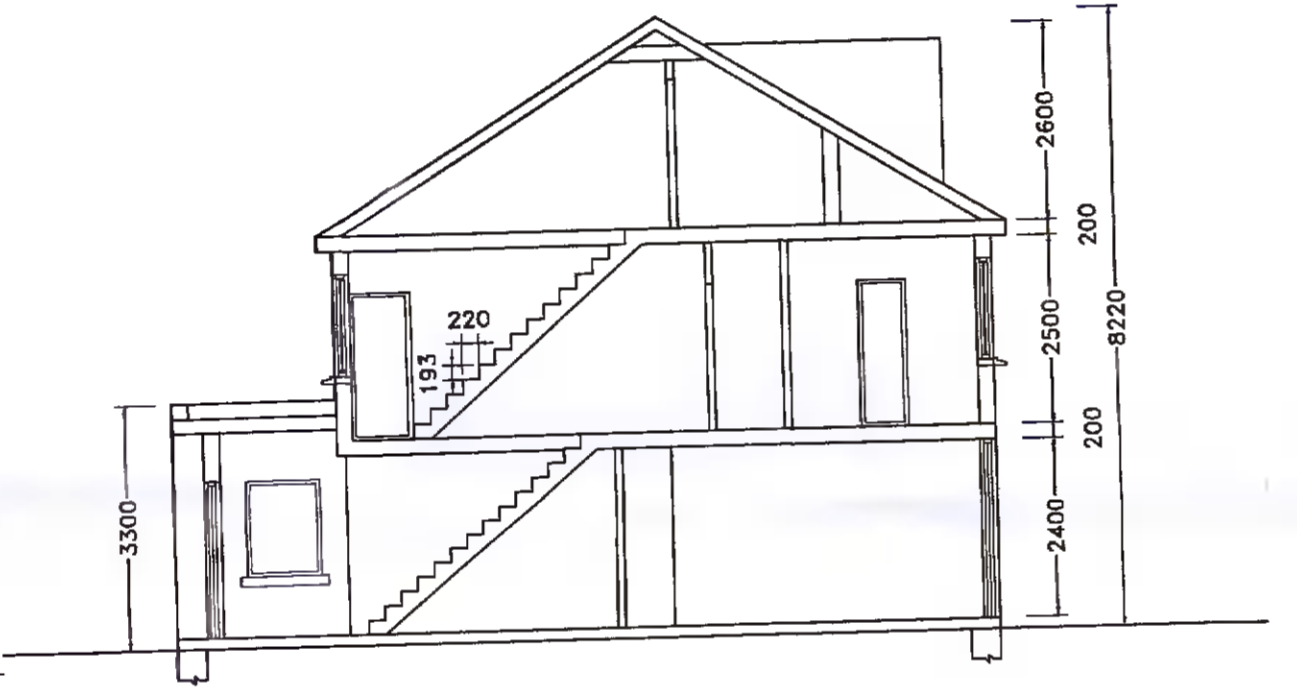
MAIN SECTION (PROPOSED) SCALE 1:100
